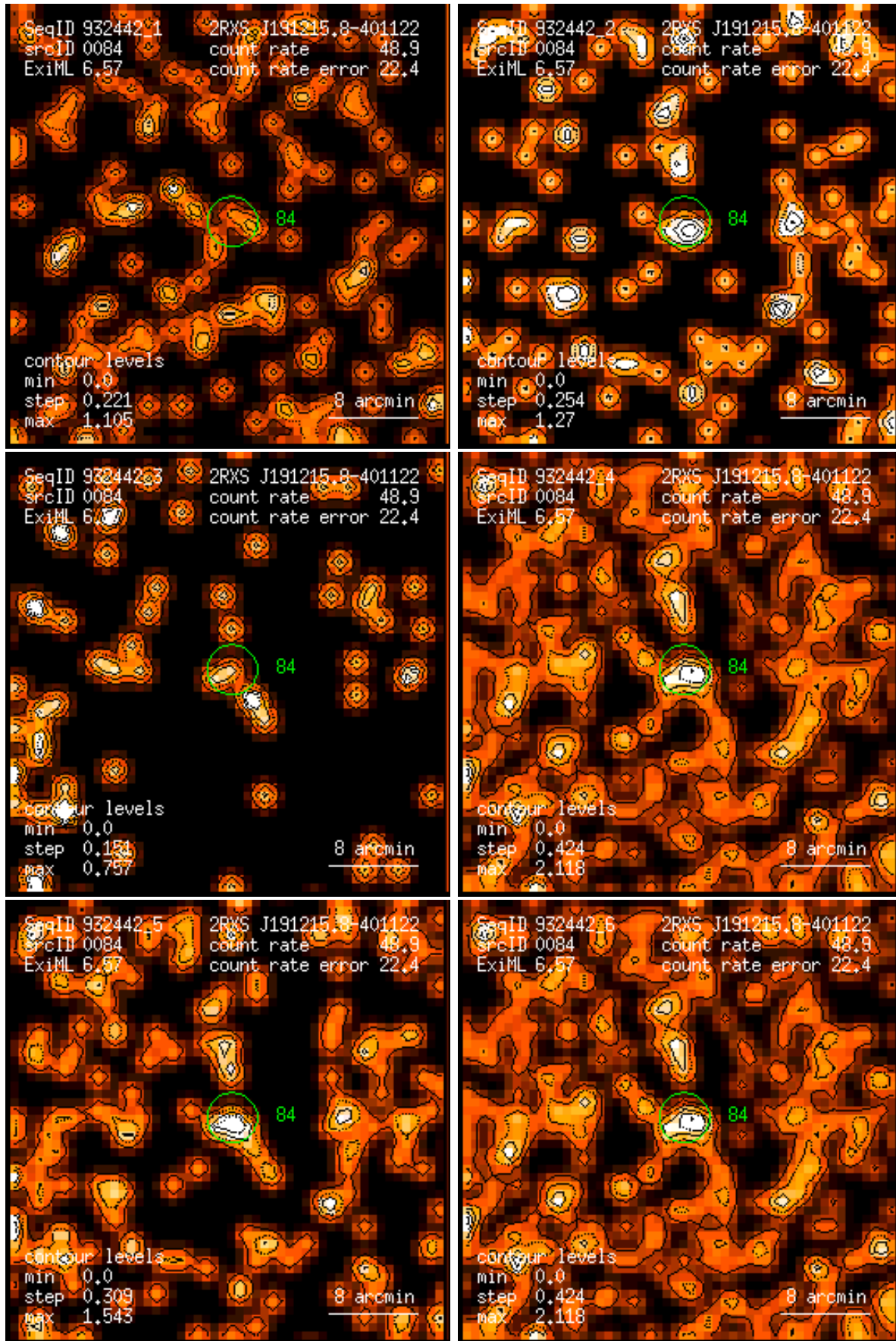
Figure 84: RASS 932442: detection 0084: band rate images, Gaussian filter: (1) PSPC channels 11 – 41, (2) 52 – 90, (3) 91 – 201, (4) 11 – 235, (5) 52 – 201, (6) 11 – 201. Broad band rates in counts/ks. Band rate contour levels in counts/ks/arcmin 2 .
