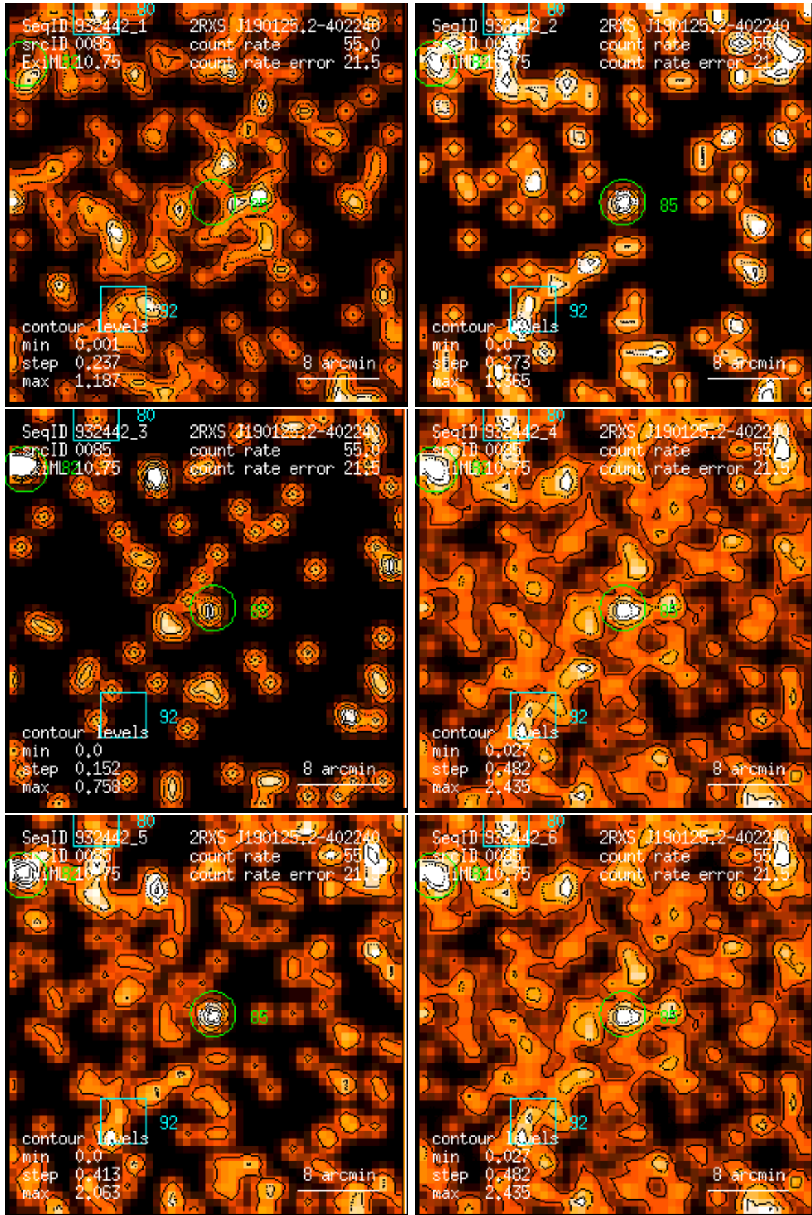
Figure 85: RASS 932442: detection 0085: band rate images, Gaussian filter: (1) PSPC channels 11 – 41, (2) 52 – 90, (3) 91 – 201, (4) 11 – 235, (5) 52 – 201, (6) 11 – 201. Broad band rates in counts/ks. Band rate contour levels in counts/ks/arcmin 2 .
