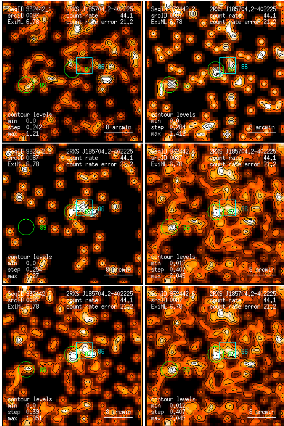
Figure 87: RASS 932442: detection 0087: band rate images, Gaussian filter: (1) PSPC channels 11 – 41, (2) 52 – 90, (3) 91 – 201, (4) 11 – 235, (5) 52 – 201, (6) 11 – 201. Broad band rates in counts/ks. Band rate contour levels in counts/ks/arcmin 2 .
