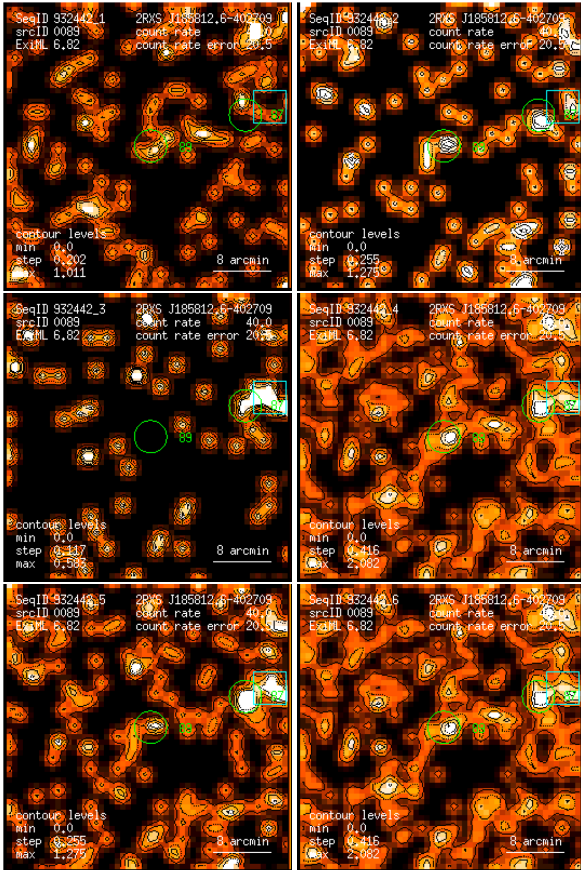
Figure 89: RASS 932442: detection 0089: band rate images, Gaussian filter: (1) PSPC channels 11 – 41, (2) 52 – 90, (3) 91 – 201, (4) 11 – 235, (5) 52 – 201, (6) 11 – 201. Broad band rates in counts/ks. Band rate contour levels in counts/ks/arcmin 2 .
