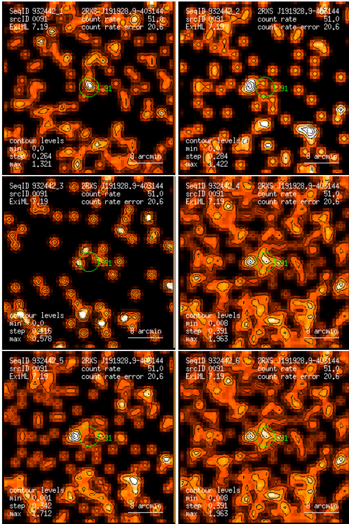
Figure 91: RASS 932442: detection 0091: band rate images, Gaussian filter: (1) PSPC channels 11 – 41, (2) 52 – 90, (3) 91 – 201, (4) 11 – 235, (5) 52 – 201, (6) 11 – 201. Broad band rates in counts/ks. Band rate contour levels in counts/ks/arcmin 2 .
