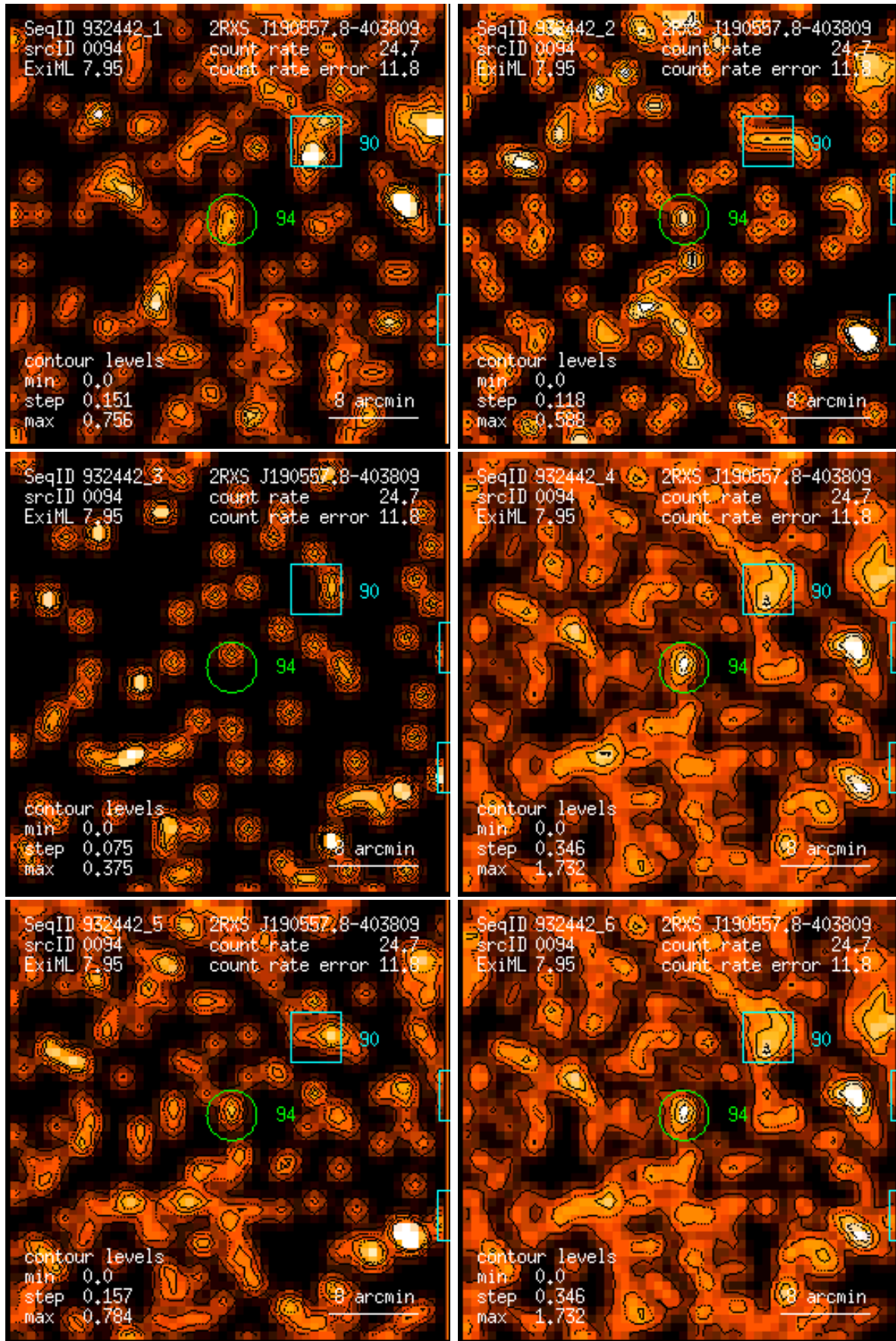
Figure 94: RASS 932442: detection 0094: band rate images, Gaussian filter: (1) PSPC channels 11 – 41, (2) 52 – 90, (3) 91 – 201, (4) 11 – 235, (5) 52 – 201, (6) 11 – 201. Broad band rates in counts/ks. Band rate contour levels in counts/ks/arcmin 2 .
