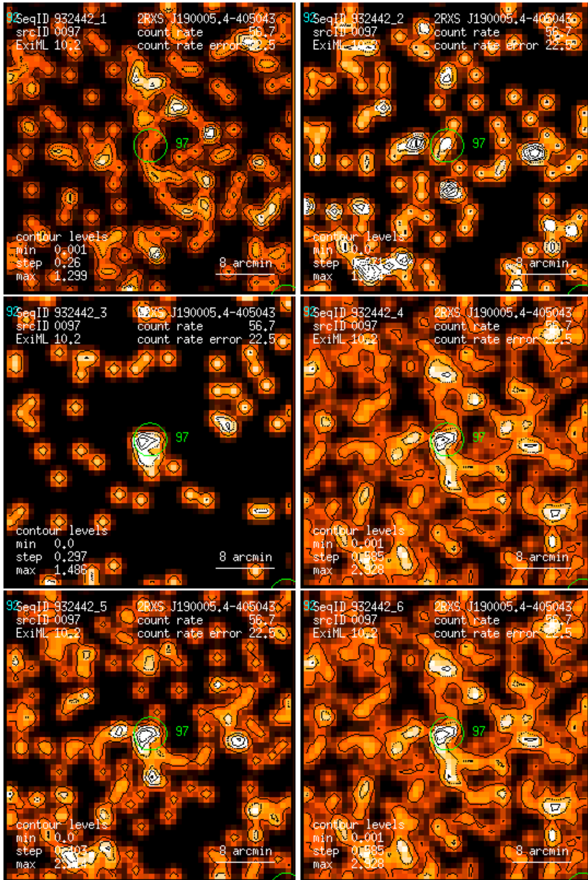
Figure 97: RASS 932442: detection 0097: band rate images, Gaussian filter: (1) PSPC channels 11 – 41, (2) 52 – 90, (3) 91 – 201, (4) 11 – 235, (5) 52 – 201, (6) 11 – 201. Broad band rates in counts/ks. Band rate contour levels in counts/ks/arcmin 2 .
