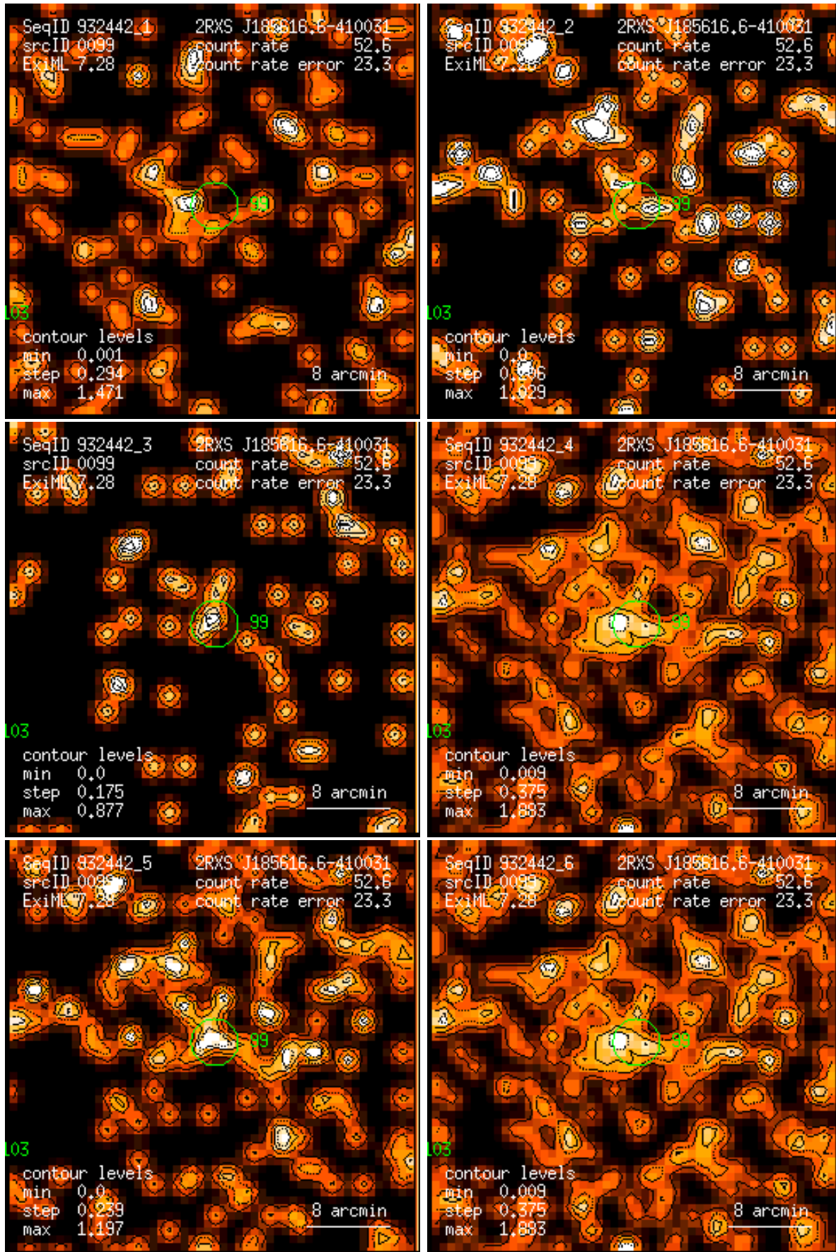
Figure 99: RASS 932442: detection 0099: band rate images, Gaussian filter: (1) PSPC channels 11 – 41, (2) 52 – 90, (3) 91 – 201, (4) 11 – 235, (5) 52 – 201, (6) 11 – 201. Broad band rates in counts/ks. Band rate contour levels in counts/ks/arcmin 2 .
