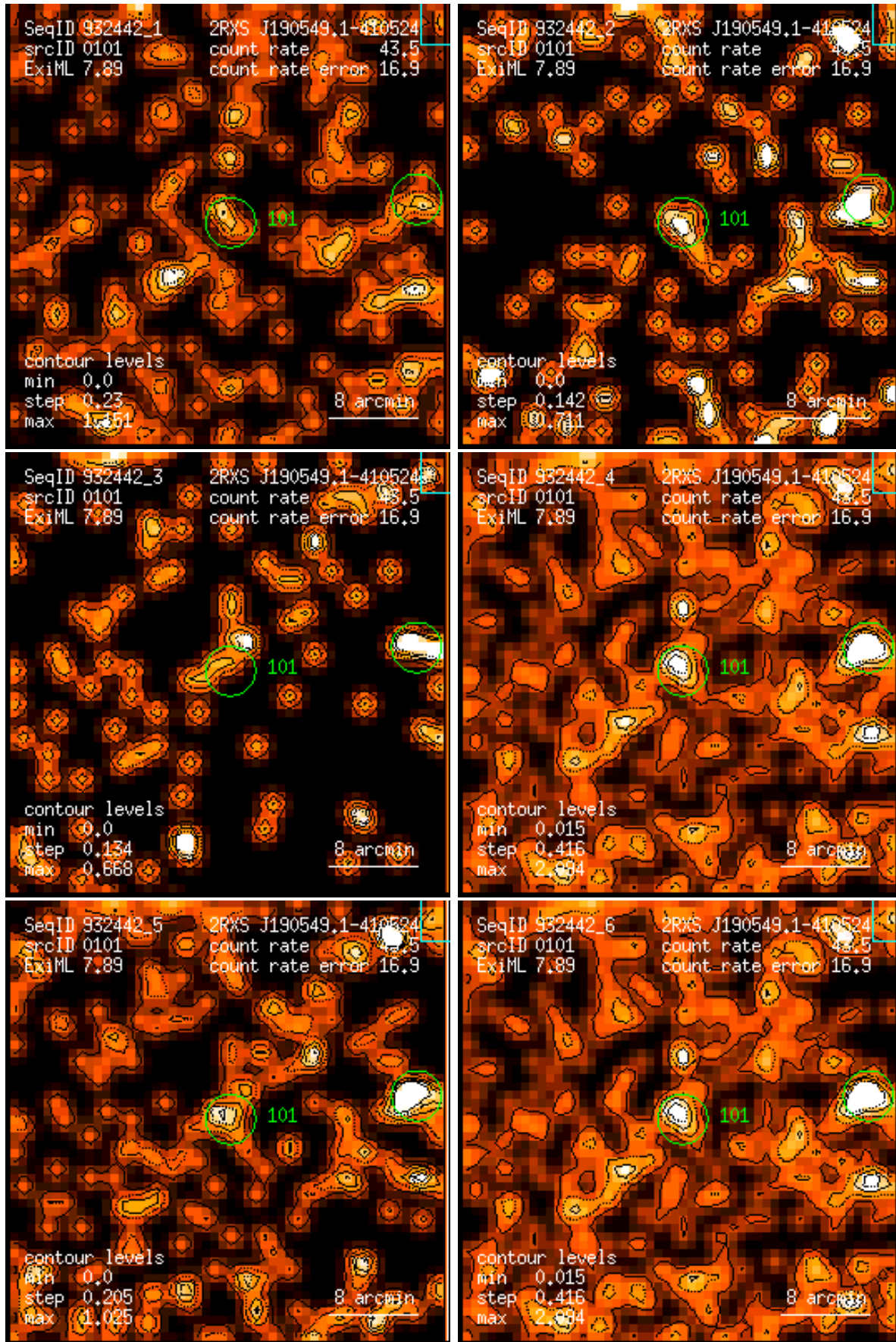
Figure 101: RASS 932442: detection 0101: band rate images, Gaussian filter: (1) PSPC channels 11 – 41, (2) 52 – 90, (3) 91 – 201, (4) 11 – 235, (5) 52 – 201, (6) 11 – 201. Broad band rates in counts/ks. Band rate contour levels in counts/ks/arcmin 2 .
