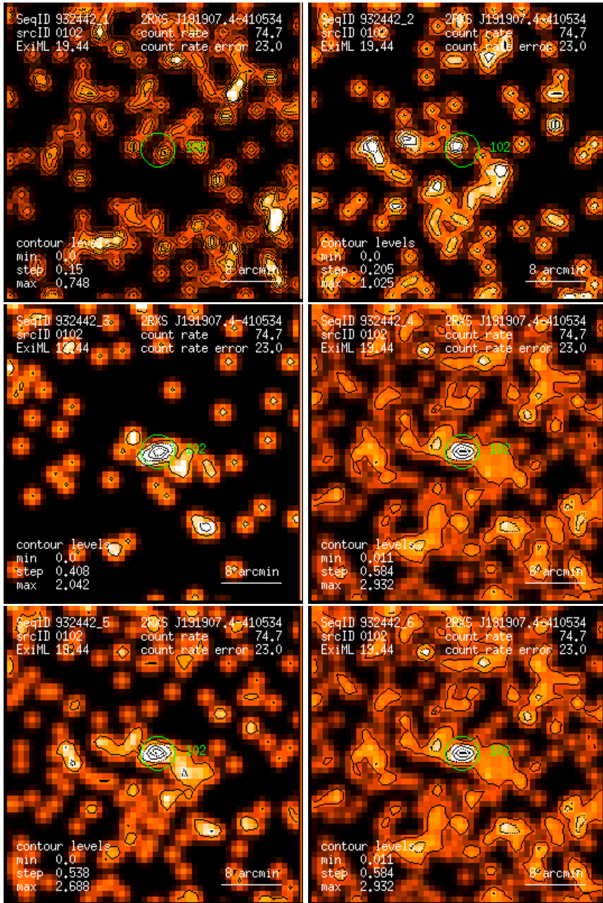
Figure 102: RASS 932442: detection 0102: band rate images, Gaussian filter: (1) PSPC channels 11 – 41, (2) 52 – 90, (3) 91 – 201, (4) 11 – 235, (5) 52 – 201, (6) 11 – 201. Broad band rates in counts/ks. Band rate contour levels in counts/ks/arcmin 2 .
