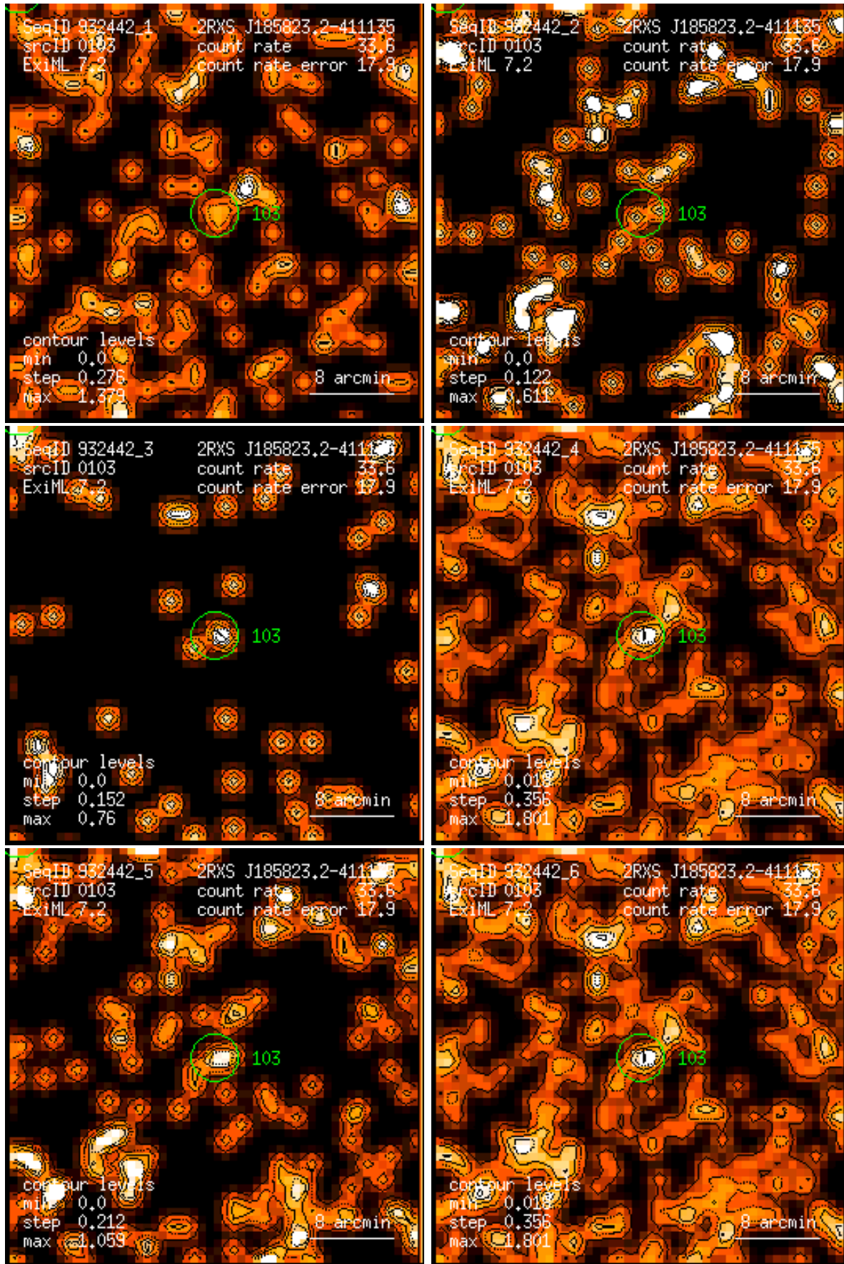
Figure 103: RASS 932442: detection 0103: band rate images, Gaussian filter: (1) PSPC channels 11 – 41, (2) 52 – 90, (3) 91 – 201, (4) 11 – 235, (5) 52 – 201, (6) 11 – 201. Broad band rates in counts/ks. Band rate contour levels in counts/ks/arcmin 2 .
