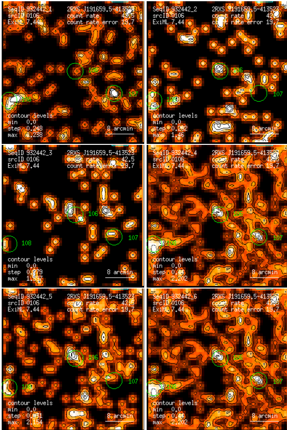
Figure 106: RASS 932442: detection 0106: band rate images, Gaussian filter: (1) PSPC channels 11 – 41, (2) 52 – 90, (3) 91 – 201, (4) 11 – 235, (5) 52 – 201, (6) 11 – 201. Broad band rates in counts/ks. Band rate contour levels in counts/ks/arcmin 2 .
