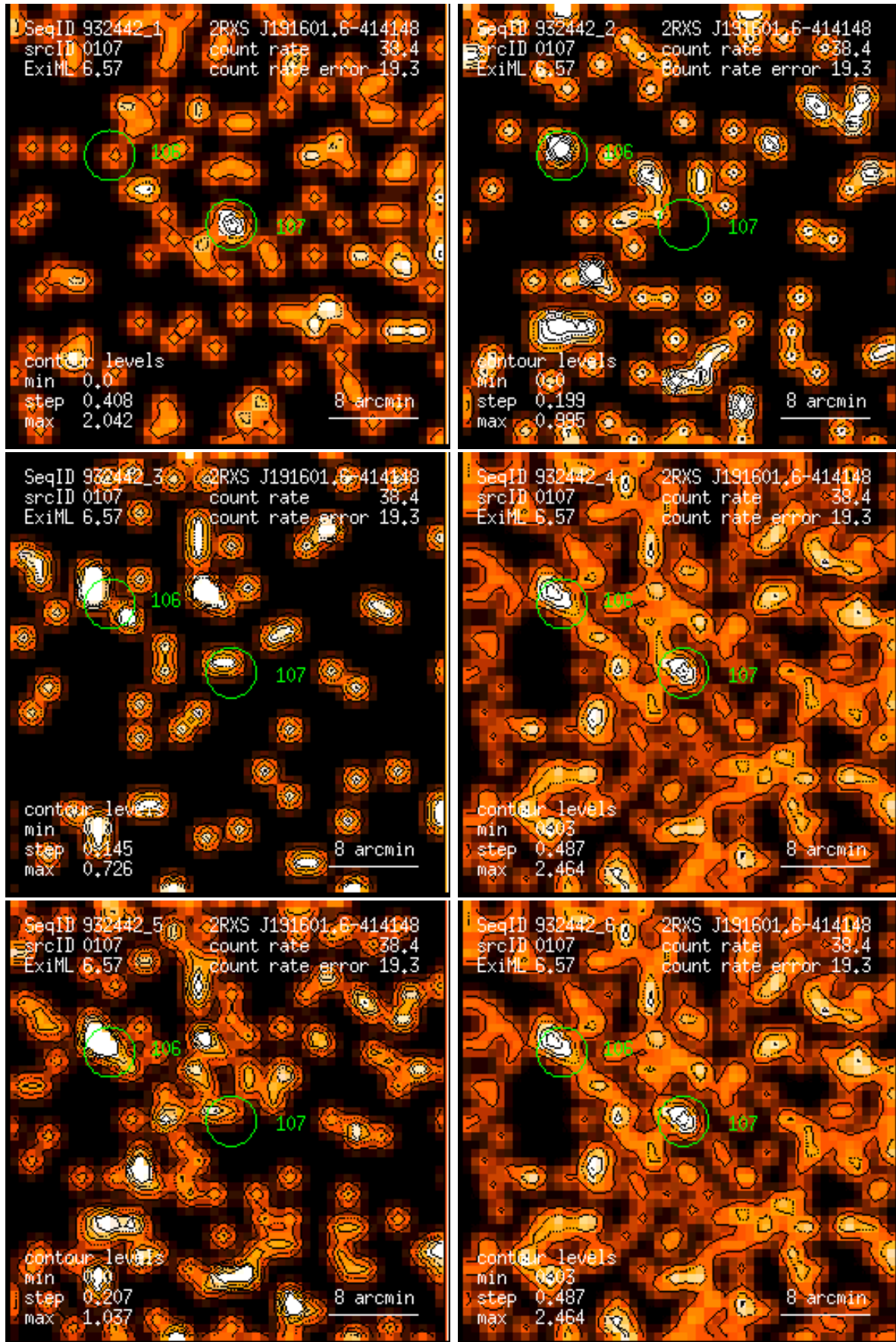
Figure 107: RASS 932442: detection 0107: band rate images, Gaussian filter: (1) PSPC channels 11 – 41, (2) 52 – 90, (3) 91 – 201, (4) 11 – 235, (5) 52 – 201, (6) 11 – 201. Broad band rates in counts/ks. Band rate contour levels in counts/ks/arcmin 2 .
