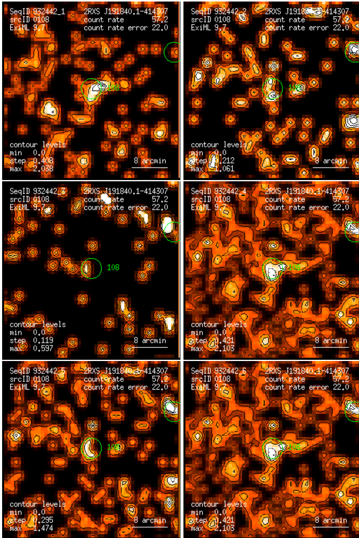
Figure 108: RASS 932442: detection 0108: band rate images, Gaussian filter: (1) PSPC channels 11 – 41, (2) 52 – 90, (3) 91 – 201, (4) 11 – 235, (5) 52 – 201, (6) 11 – 201. Broad band rates in counts/ks. Band rate contour levels in counts/ks/arcmin 2 .
