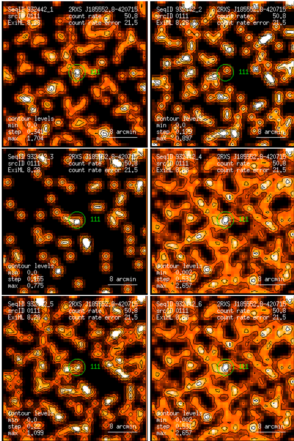
Figure 111: RASS 932442: detection 0111: band rate images, Gaussian filter: (1) PSPC channels 11 – 41, (2) 52 – 90, (3) 91 – 201, (4) 11 – 235, (5) 52 – 201, (6) 11 – 201. Broad band rates in counts/ks. Band rate contour levels in counts/ks/arcmin 2 .
