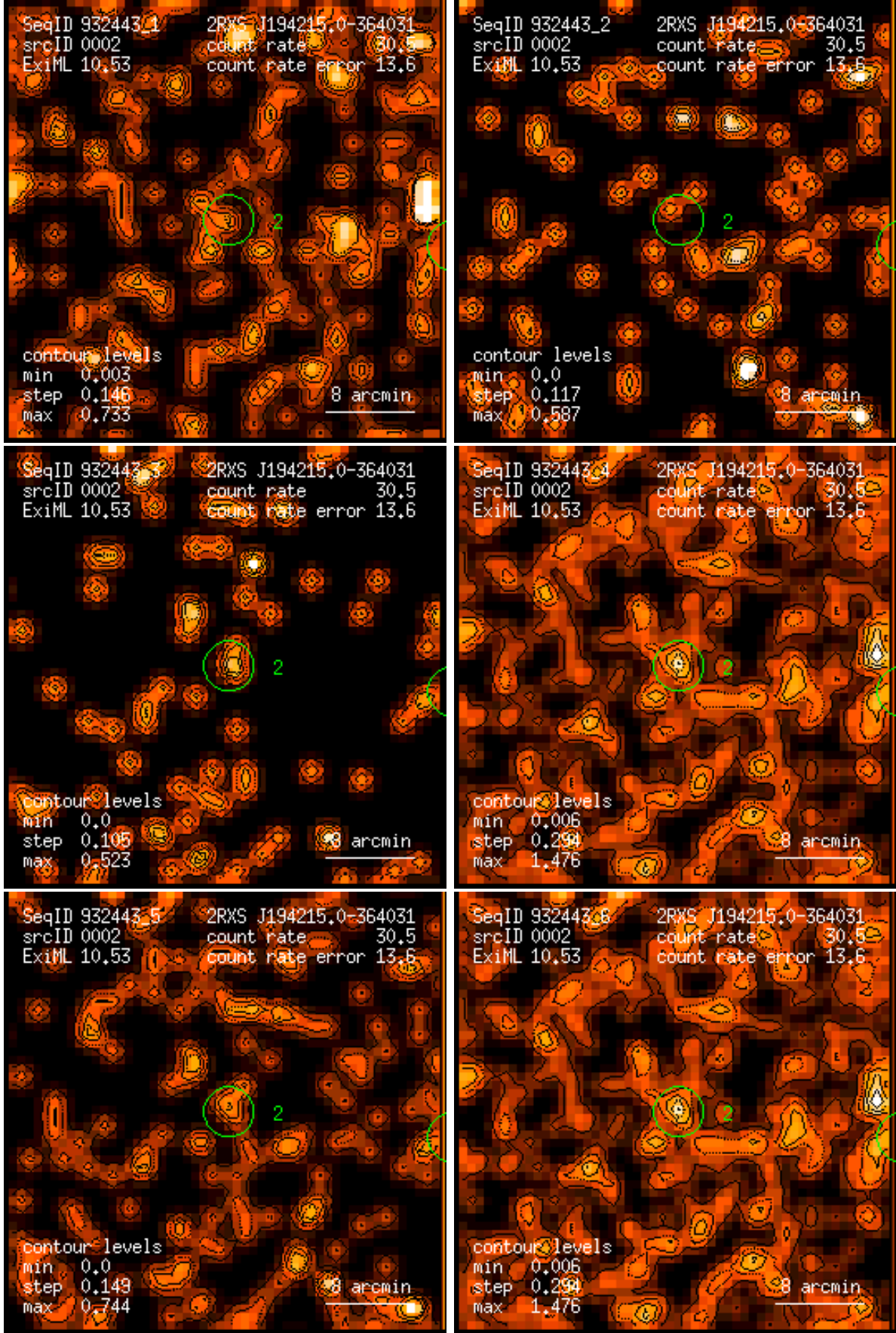
Figure 2: RASS 932443: detection 0002: band rate images, Gaussian filter: (1) PSPC channels 11 – 41, (2) 52 – 90, (3) 91 – 201, (4) 11 – 235, (5) 52 – 201, (6) 11 – 201. Broad band rates in counts/ks. Band rate contour levels in counts/ks/arcmin 2 .
