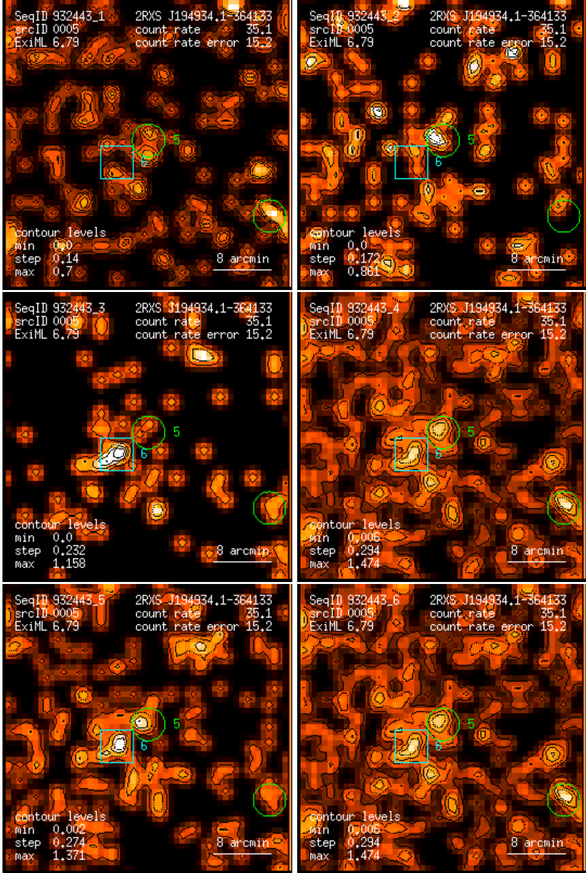
Figure 5: RASS 932443: detection 0005: band rate images, Gaussian filter: (1) PSPC channels 11 – 41, (2) 52 – 90, (3) 91 – 201, (4) 11 – 235, (5) 52 – 201, (6) 11 – 201. Broad band rates in counts/ks. Band rate contour levels in counts/ks/arcmin 2 .
