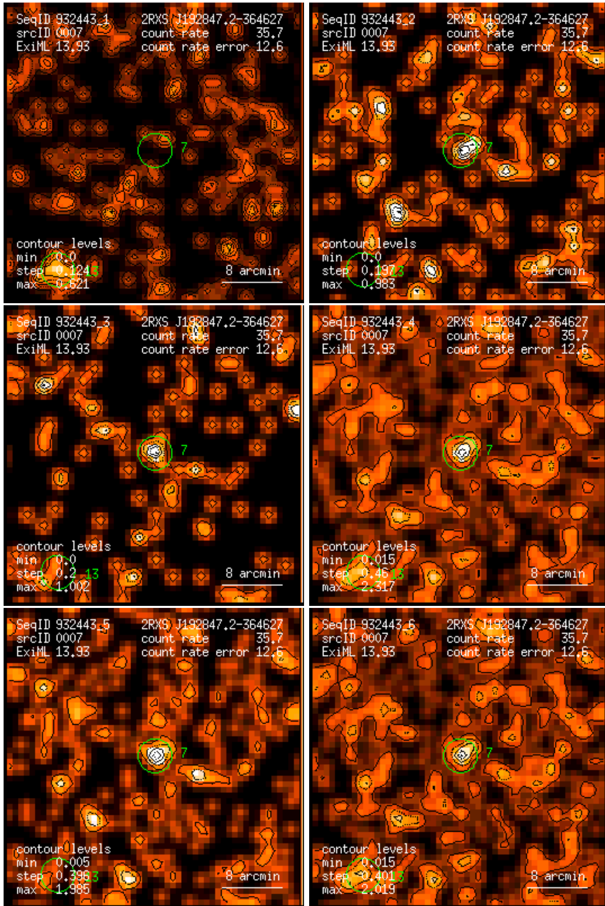
Figure 7: RASS 932443: detection 0007: band rate images, Gaussian filter: (1) PSPC channels 11 – 41, (2) 52 – 90, (3) 91 – 201, (4) 11 – 235, (5) 52 – 201, (6) 11 – 201. Broad band rates in counts/ks. Band rate contour levels in counts/ks/arcmin 2 .
