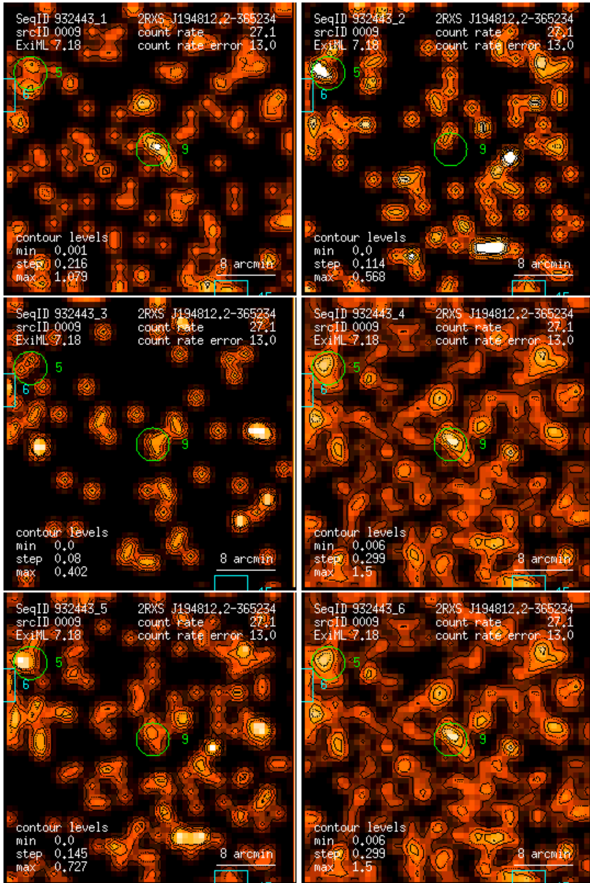
Figure 9: RASS 932443: detection 0009: band rate images, Gaussian filter: (1) PSPC channels 11 – 41, (2) 52 – 90, (3) 91 – 201, (4) 11 – 235, (5) 52 – 201, (6) 11 – 201. Broad band rates in counts/ks. Band rate contour levels in counts/ks/arcmin 2 .
