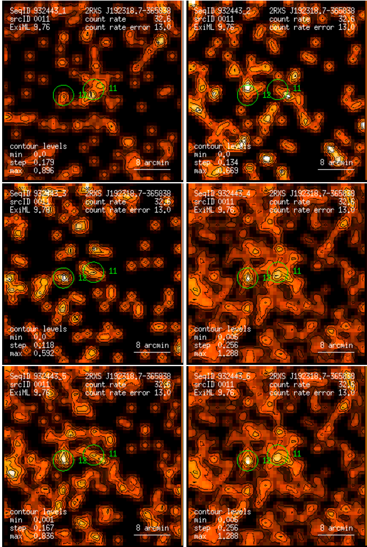
Figure 11: RASS 932443: detection 0011: band rate images, Gaussian filter: (1) PSPC channels 11 – 41, (2) 52 – 90, (3) 91 – 201, (4) 11 – 235, (5) 52 – 201, (6) 11 – 201. Broad band rates in counts/ks. Band rate contour levels in counts/ks/arcmin 2 .
