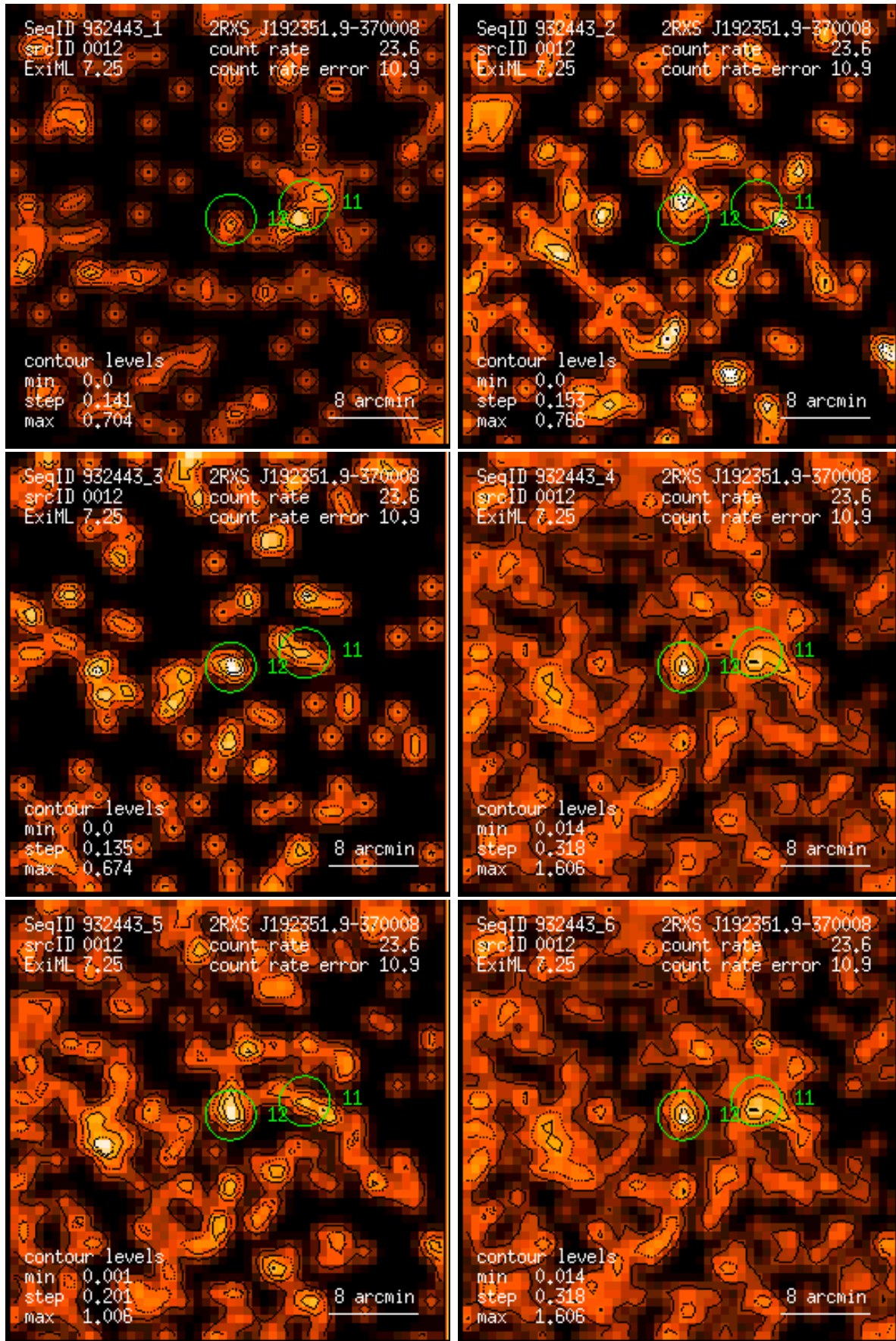
Figure 12: RASS 932443: detection 0012: band rate images, Gaussian filter: (1) PSPC channels 11 – 41, (2) 52 – 90, (3) 91 – 201, (4) 11 – 235, (5) 52 – 201, (6) 11 – 201. Broad band rates in counts/ks. Band rate contour levels in counts/ks/arcmin 2 .
