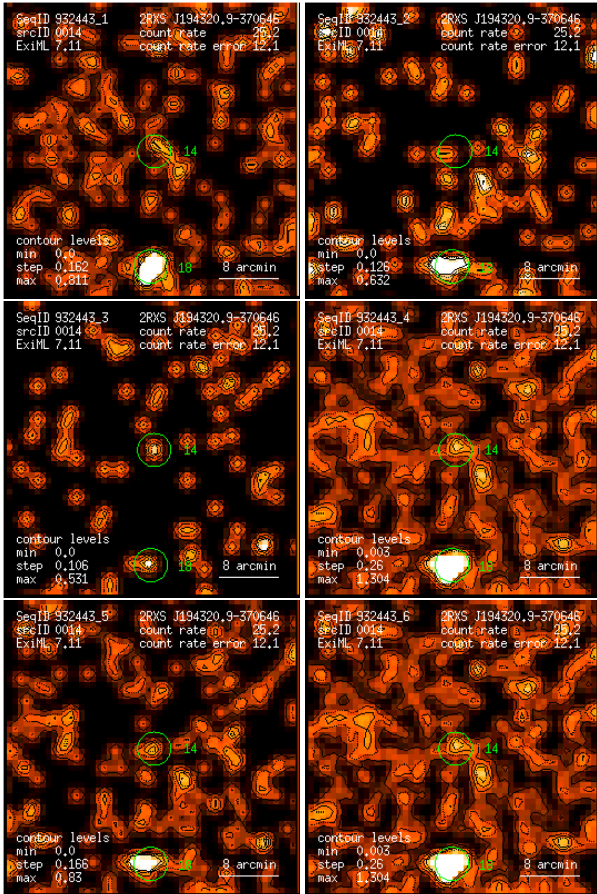
Figure 14: RASS 932443: detection 0014: band rate images, Gaussian filter: (1) PSPC channels 11 – 41, (2) 52 – 90, (3) 91 – 201, (4) 11 – 235, (5) 52 – 201, (6) 11 – 201. Broad band rates in counts/ks. Band rate contour levels in counts/ks/arcmin 2 .
