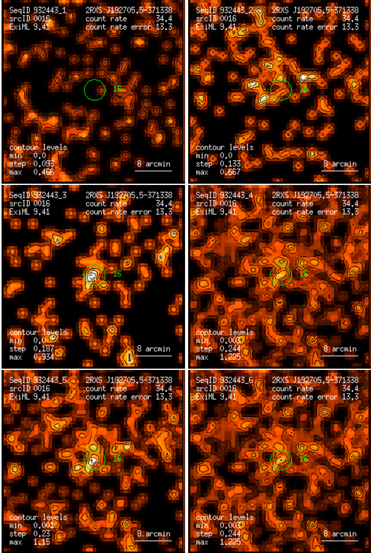
Figure 16: RASS 932443: detection 0016: band rate images, Gaussian filter: (1) PSPC channels 11 – 41, (2) 52 – 90, (3) 91 – 201, (4) 11 – 235, (5) 52 – 201, (6) 11 – 201. Broad band rates in counts/ks. Band rate contour levels in counts/ks/arcmin 2 .
