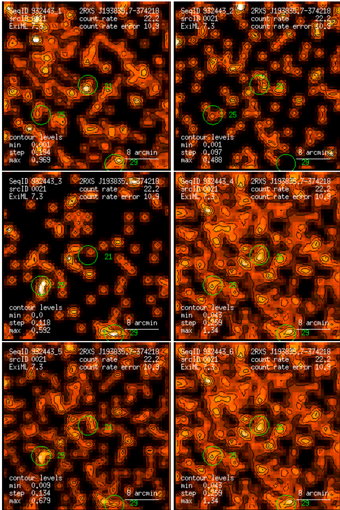
Figure 21: RASS 932443: detection 0021: band rate images, Gaussian filter: (1) PSPC channels 11 – 41, (2) 52 – 90, (3) 91 – 201, (4) 11 – 235, (5) 52 – 201, (6) 11 – 201. Broad band rates in counts/ks. Band rate contour levels in counts/ks/arcmin 2 .
