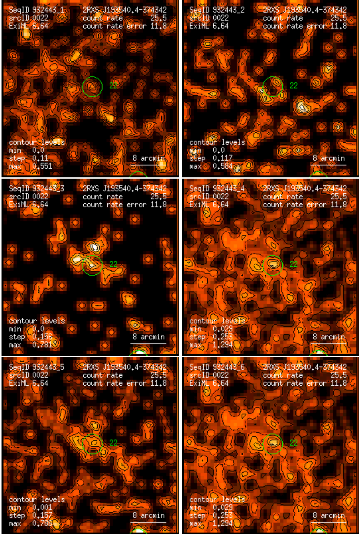
Figure 22: RASS 932443: detection 0022: band rate images, Gaussian filter: (1) PSPC channels 11 – 41, (2) 52 – 90, (3) 91 – 201, (4) 11 – 235, (5) 52 – 201, (6) 11 – 201. Broad band rates in counts/ks. Band rate contour levels in counts/ks/arcmin 2 .
