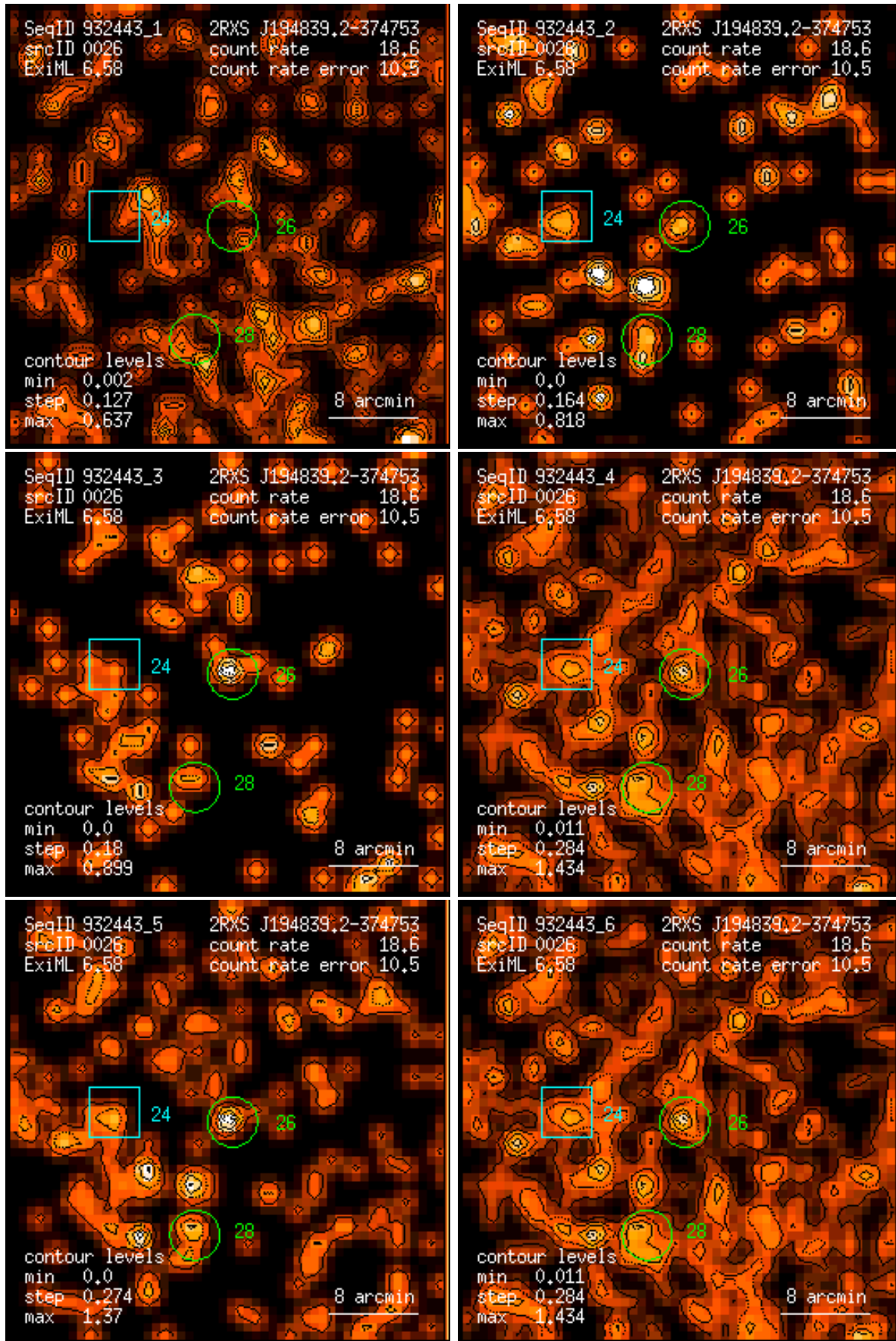
Figure 26: RASS 932443: detection 0026: band rate images, Gaussian filter: (1) PSPC channels 11 – 41, (2) 52 – 90, (3) 91 – 201, (4) 11 – 235, (5) 52 – 201, (6) 11 – 201. Broad band rates in counts/ks. Band rate contour levels in counts/ks/arcmin 2 .
