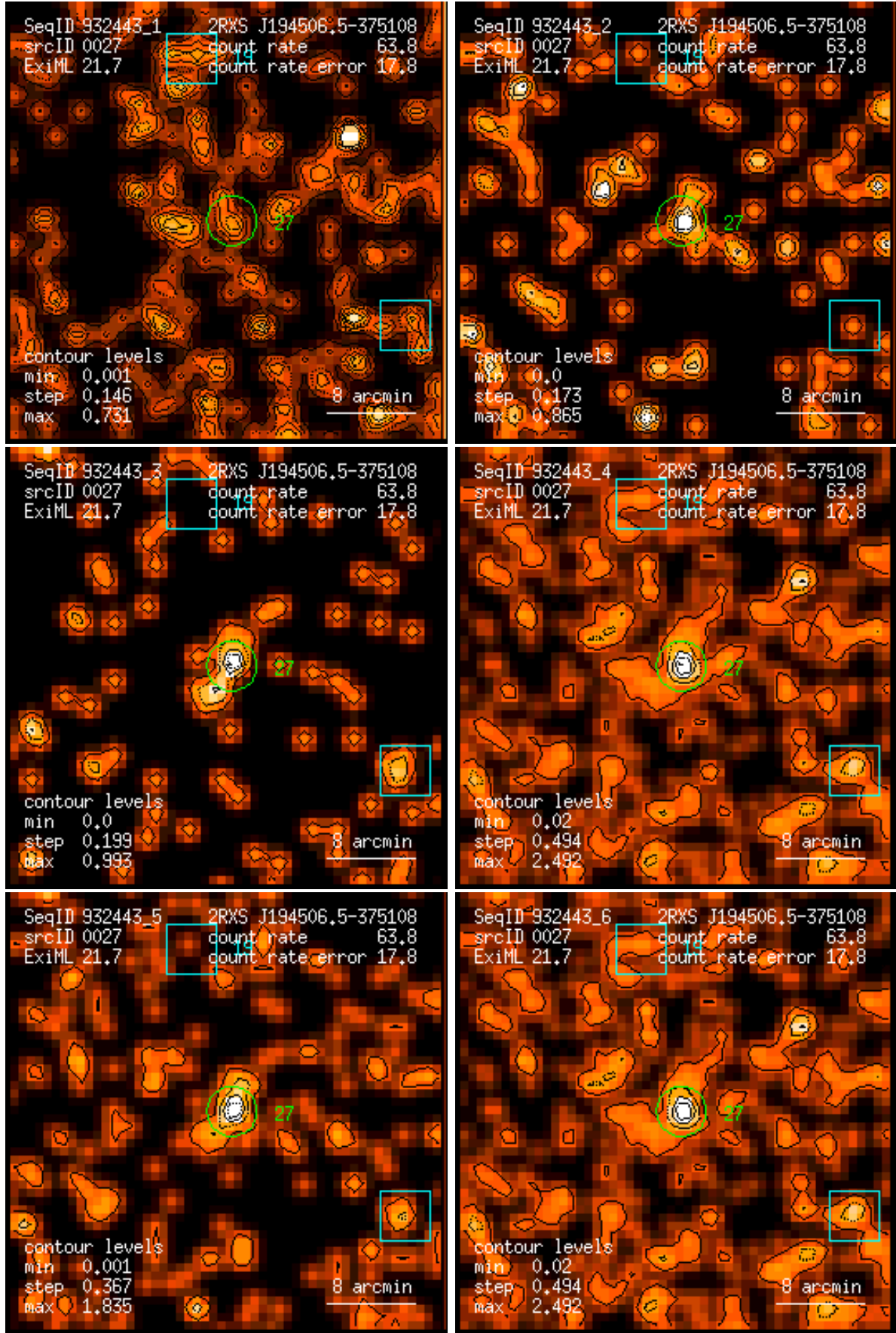
Figure 27: RASS 932443: detection 0027: band rate images, Gaussian filter: (1) PSPC channels 11 – 41, (2) 52 – 90, (3) 91 – 201, (4) 11 – 235, (5) 52 – 201, (6) 11 – 201. Broad band rates in counts/ks. Band rate contour levels in counts/ks/arcmin 2 .
