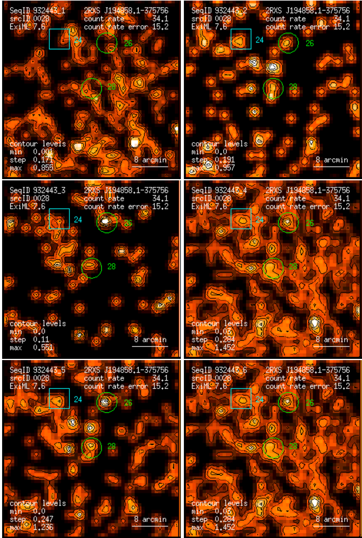
Figure 28: RASS 932443: detection 0028: band rate images, Gaussian filter: (1) PSPC channels 11 – 41, (2) 52 – 90, (3) 91 – 201, (4) 11 – 235, (5) 52 – 201, (6) 11 – 201. Broad band rates in counts/ks. Band rate contour levels in counts/ks/arcmin 2 .
