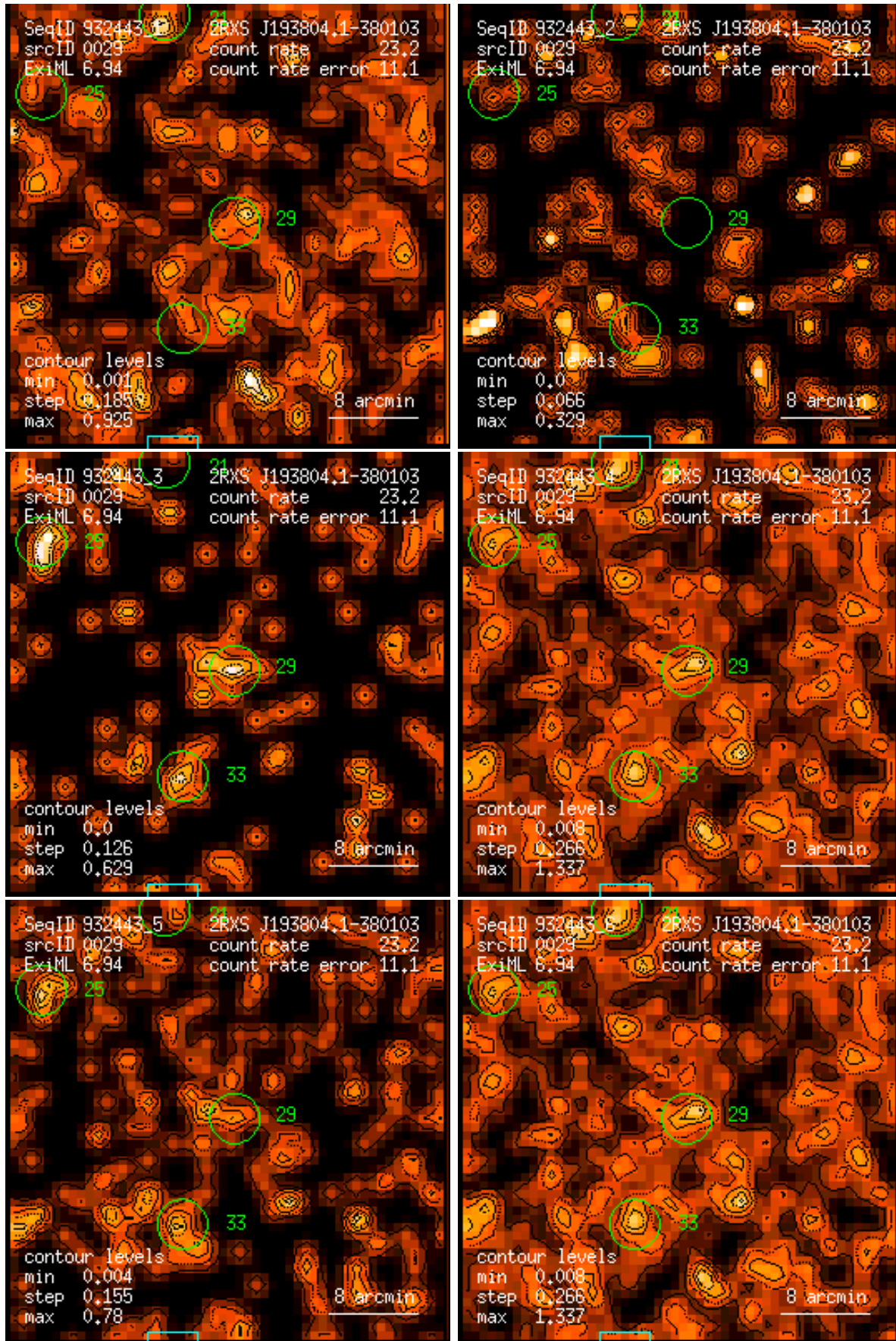
Figure 29: RASS 932443: detection 0029: band rate images, Gaussian filter: (1) PSPC channels 11 – 41, (2) 52 – 90, (3) 91 – 201, (4) 11 – 235, (5) 52 – 201, (6) 11 – 201. Broad band rates in counts/ks. Band rate contour levels in counts/ks/arcmin 2 .
