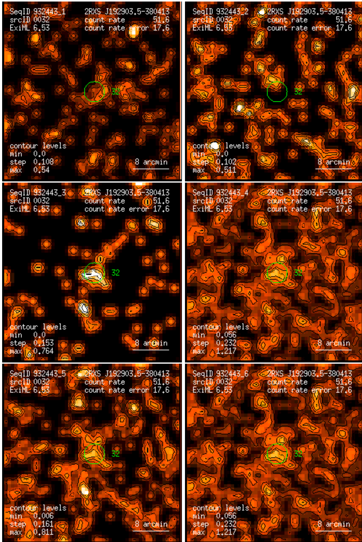
Figure 32: RASS 932443: detection 0032: band rate images, Gaussian filter: (1) PSPC channels 11 – 41, (2) 52 – 90, (3) 91 – 201, (4) 11 – 235, (5) 52 – 201, (6) 11 – 201. Broad band rates in counts/ks. Band rate contour levels in counts/ks/arcmin 2 .
