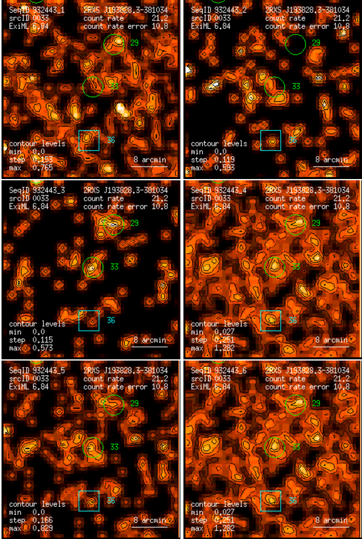
Figure 33: RASS 932443: detection 0033: band rate images, Gaussian filter: (1) PSPC channels 11 – 41, (2) 52 – 90, (3) 91 – 201, (4) 11 – 235, (5) 52 – 201, (6) 11 – 201. Broad band rates in counts/ks. Band rate contour levels in counts/ks/arcmin 2 .
