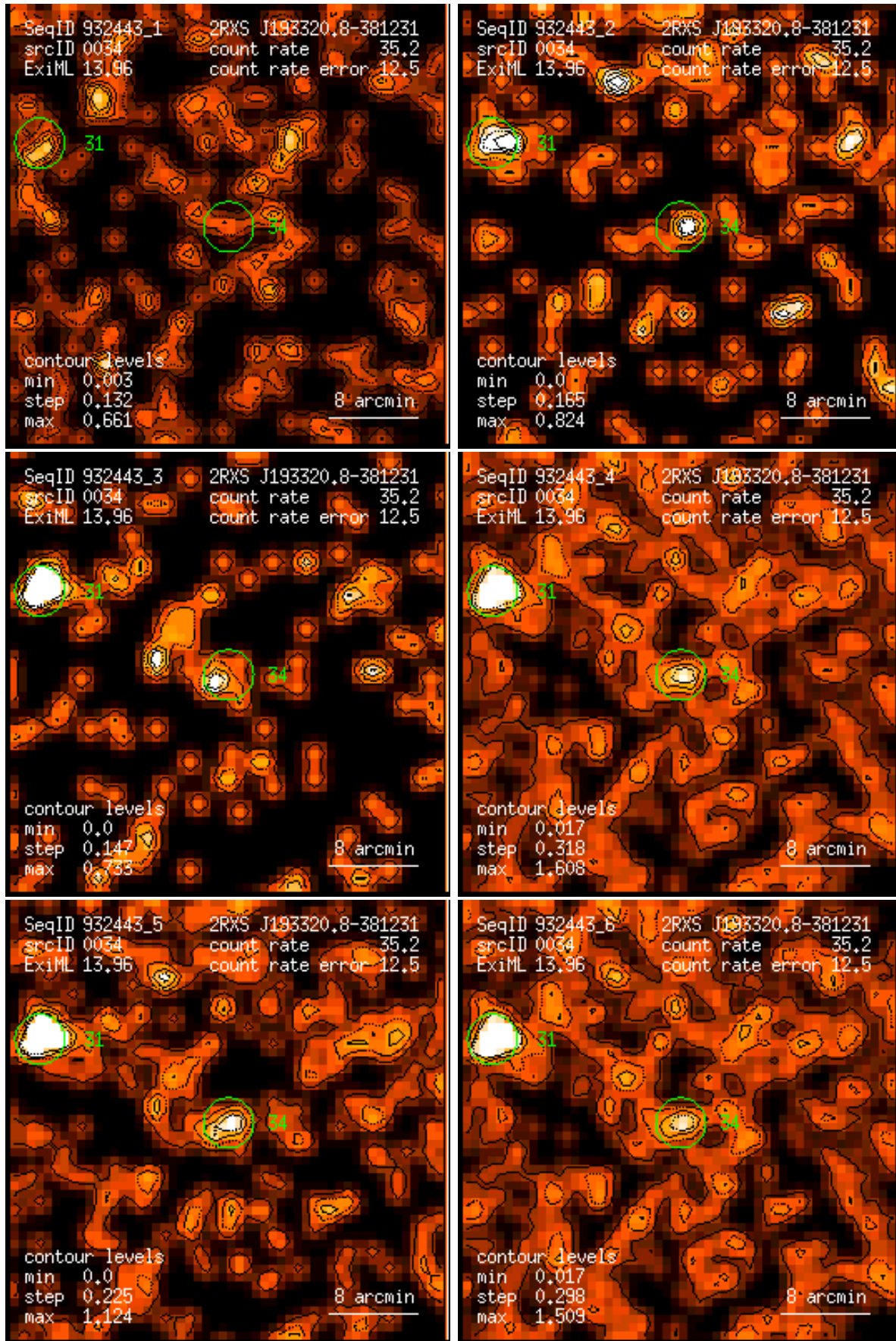
Figure 34: RASS 932443: detection 0034: band rate images, Gaussian filter: (1) PSPC channels 11 – 41, (2) 52 – 90, (3) 91 – 201, (4) 11 – 235, (5) 52 – 201, (6) 11 – 201. Broad band rates in counts/ks. Band rate contour levels in counts/ks/arcmin 2 .
