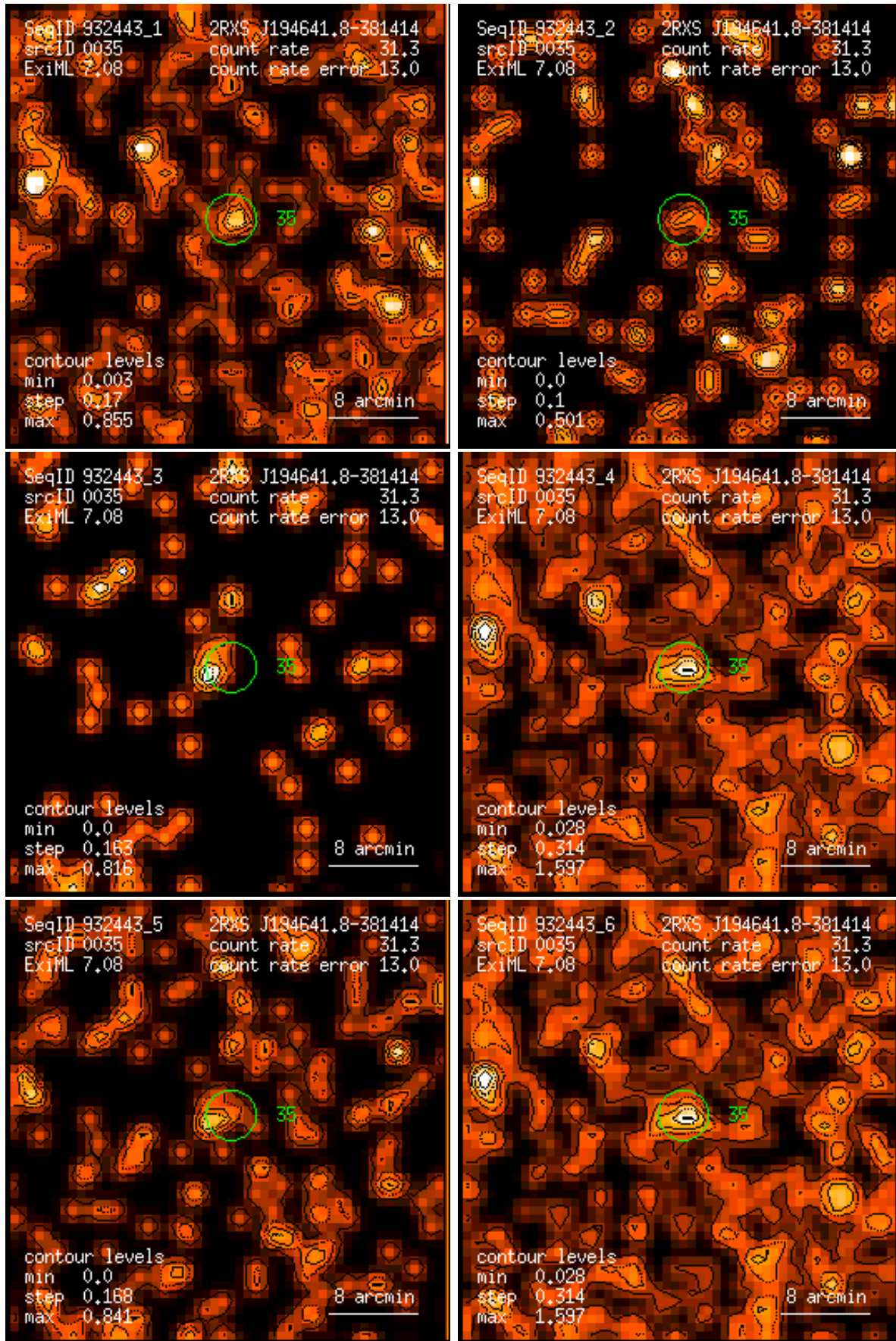
Figure 35: RASS 932443: detection 0035: band rate images, Gaussian filter: (1) PSPC channels 11 – 41, (2) 52 – 90, (3) 91 – 201, (4) 11 – 235, (5) 52 – 201, (6) 11 – 201. Broad band rates in counts/ks. Band rate contour levels in counts/ks/arcmin 2 .
