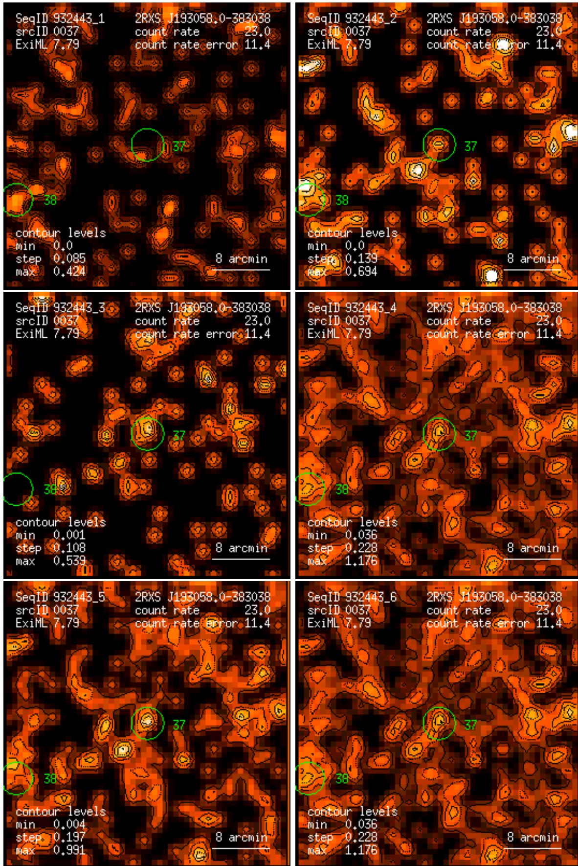
Figure 37: RASS 932443: detection 0037: band rate images, Gaussian filter: (1) PSPC channels 11 – 41, (2) 52 – 90, (3) 91 – 201, (4) 11 – 235, (5) 52 – 201, (6) 11 – 201. Broad band rates in counts/ks. Band rate contour levels in counts/ks/arcmin 2 .
