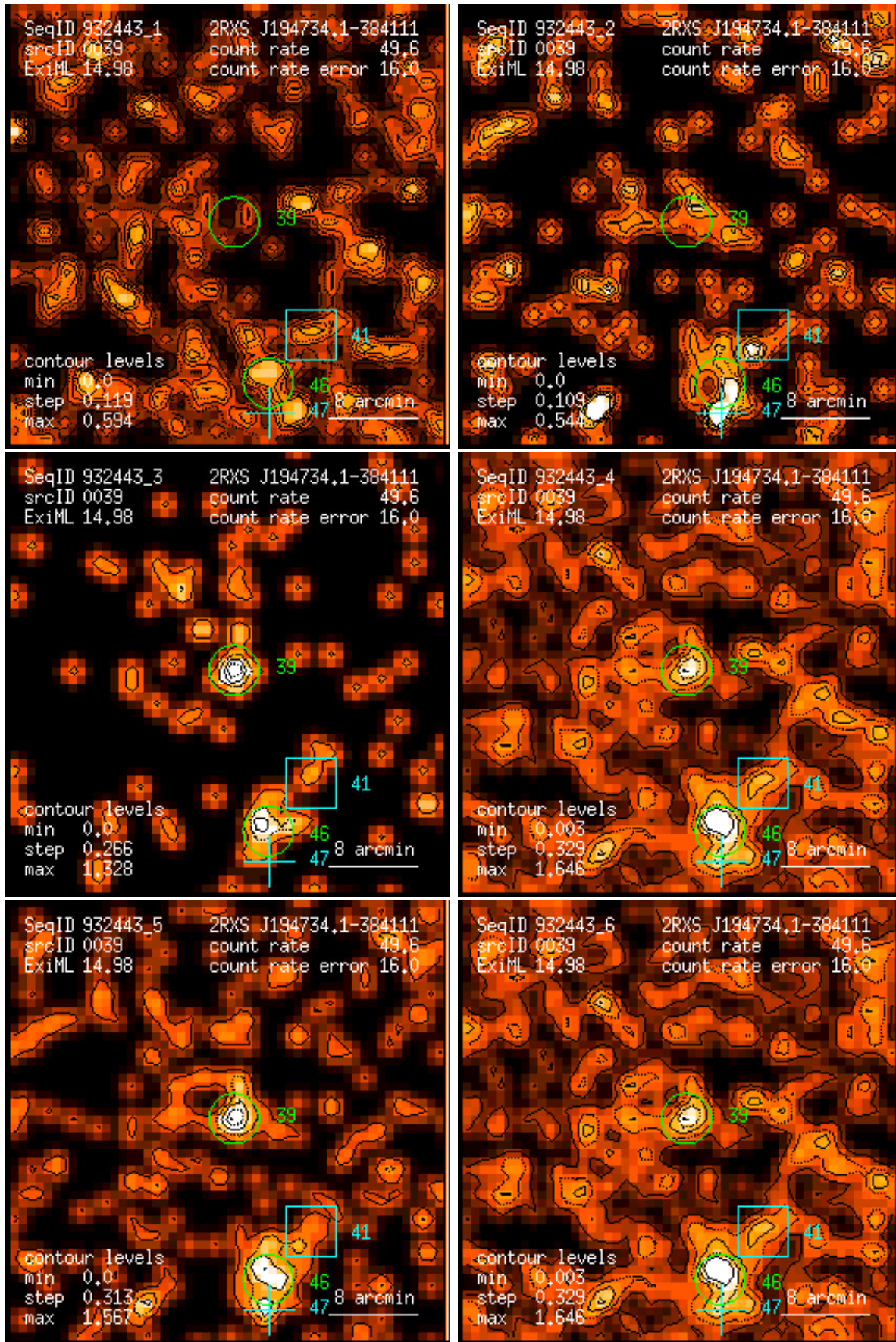
Figure 39: RASS 932443: detection 0039: band rate images, Gaussian filter: (1) PSPC channels 11 – 41, (2) 52 – 90, (3) 91 – 201, (4) 11 – 235, (5) 52 – 201, (6) 11 – 201. Broad band rates in counts/ks. Band rate contour levels in counts/ks/arcmin 2 .
