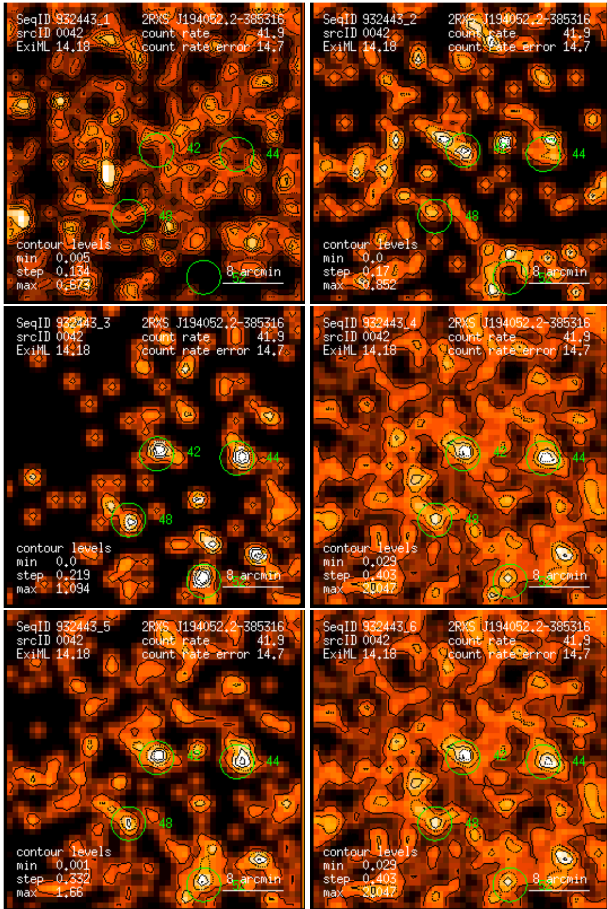
Figure 42: RASS 932443: detection 0042: band rate images, Gaussian filter: (1) PSPC channels 11 – 41, (2) 52 – 90, (3) 91 – 201, (4) 11 – 235, (5) 52 – 201, (6) 11 – 201. Broad band rates in counts/ks. Band rate contour levels in counts/ks/arcmin 2 .
