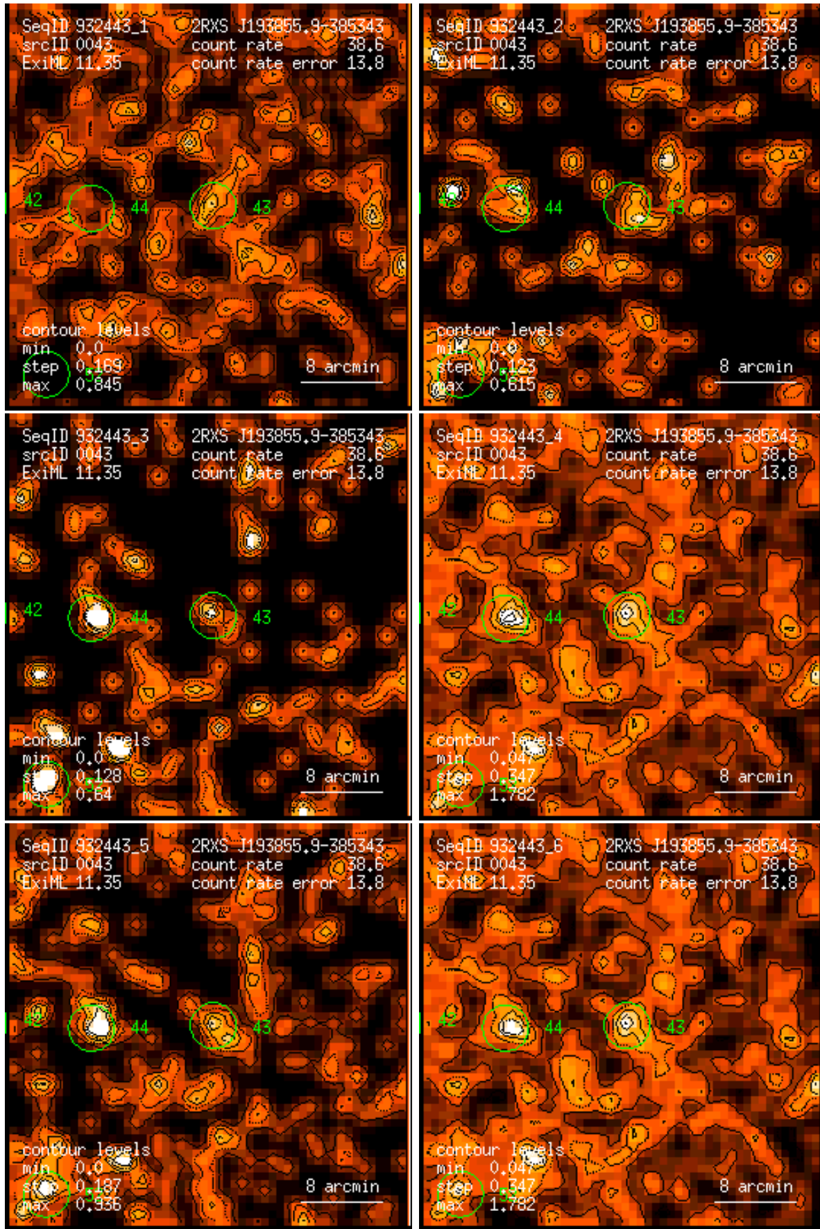
Figure 43: RASS 932443: detection 0043: band rate images, Gaussian filter: (1) PSPC channels 11 – 41, (2) 52 – 90, (3) 91 – 201, (4) 11 – 235, (5) 52 – 201, (6) 11 – 201. Broad band rates in counts/ks. Band rate contour levels in counts/ks/arcmin 2 .
