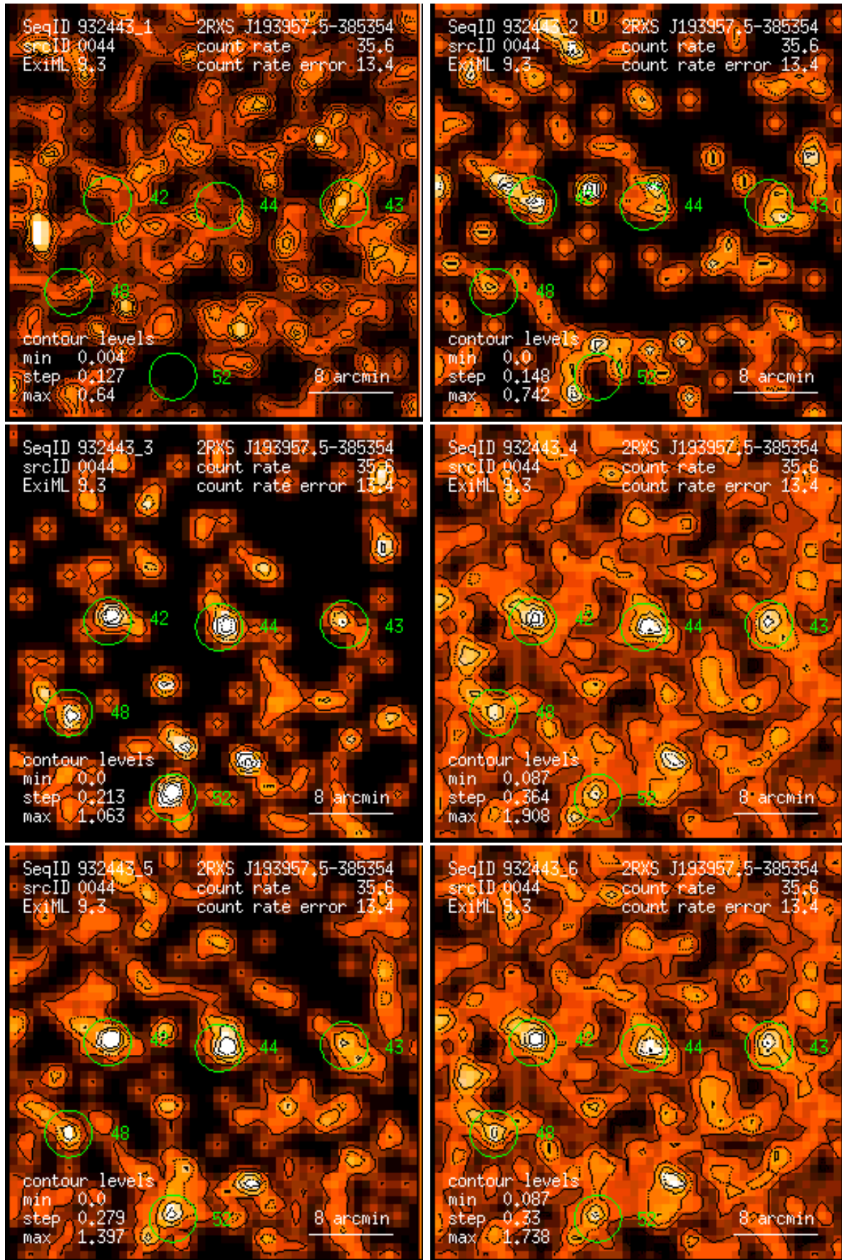
Figure 44: RASS 932443: detection 0044: band rate images, Gaussian filter: (1) PSPC channels 11 – 41, (2) 52 – 90, (3) 91 – 201, (4) 11 – 235, (5) 52 – 201, (6) 11 – 201. Broad band rates in counts/ks. Band rate contour levels in counts/ks/arcmin 2 .
