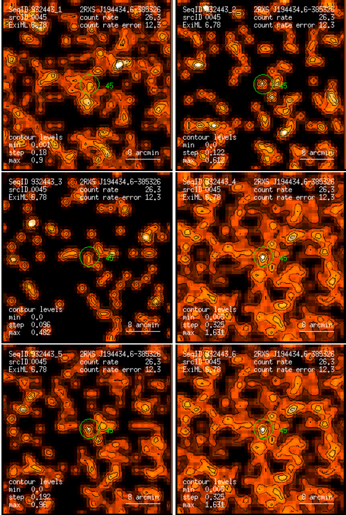
Figure 45: RASS 932443: detection 0045: band rate images, Gaussian filter: (1) PSPC channels 11 – 41, (2) 52 – 90, (3) 91 – 201, (4) 11 – 235, (5) 52 – 201, (6) 11 – 201. Broad band rates in counts/ks. Band rate contour levels in counts/ks/arcmin 2 .
