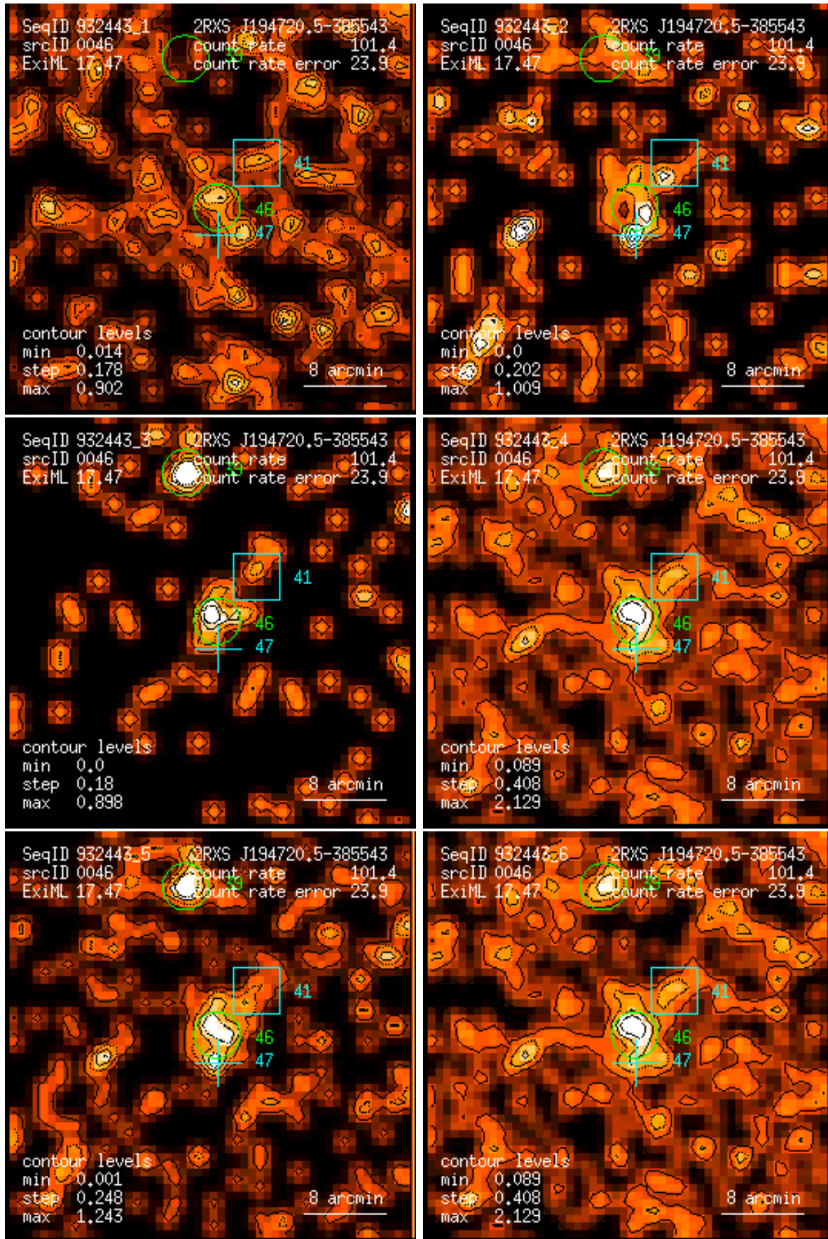
Figure 46: RASS 932443: detection 0046: band rate images, Gaussian filter: (1) PSPC channels 11 – 41, (2) 52 – 90, (3) 91 – 201, (4) 11 – 235, (5) 52 – 201, (6) 11 – 201. Broad band rates in counts/ks. Band rate contour levels in counts/ks/arcmin 2 .
