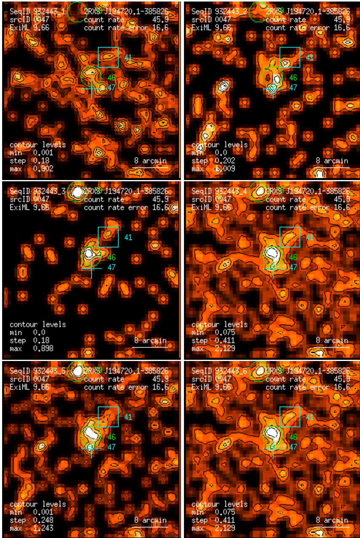
Figure 47: RASS 932443: detection 0047: band rate images, Gaussian filter: (1) PSPC channels 11 – 41, (2) 52 – 90, (3) 91 – 201, (4) 11 – 235, (5) 52 – 201, (6) 11 – 201. Broad band rates in counts/ks. Band rate contour levels in counts/ks/arcmin 2 .
