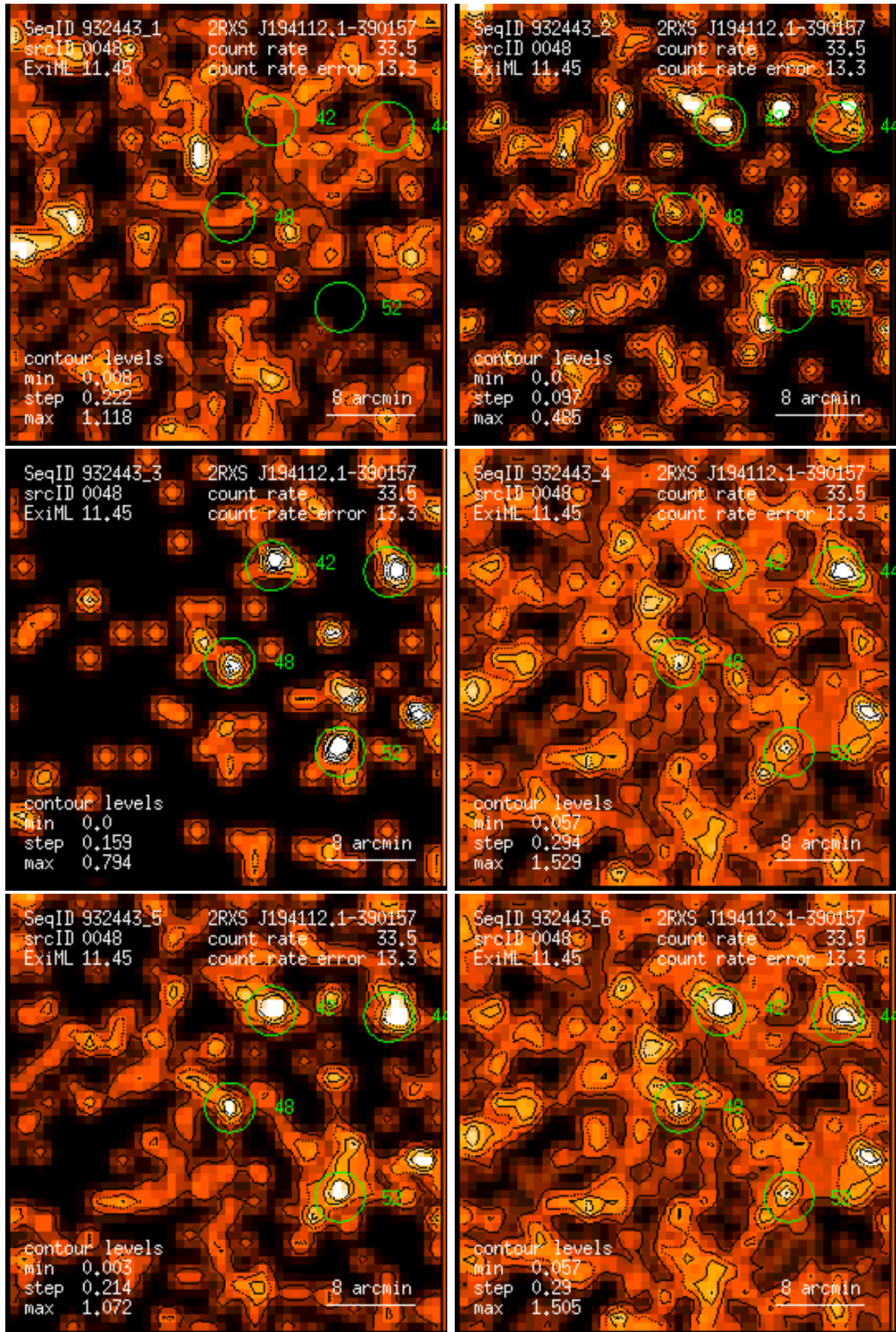
Figure 48: RASS 932443: detection 0048: band rate images, Gaussian filter: (1) PSPC channels 11 – 41, (2) 52 – 90, (3) 91 – 201, (4) 11 – 235, (5) 52 – 201, (6) 11 – 201. Broad band rates in counts/ks. Band rate contour levels in counts/ks/arcmin 2 .
