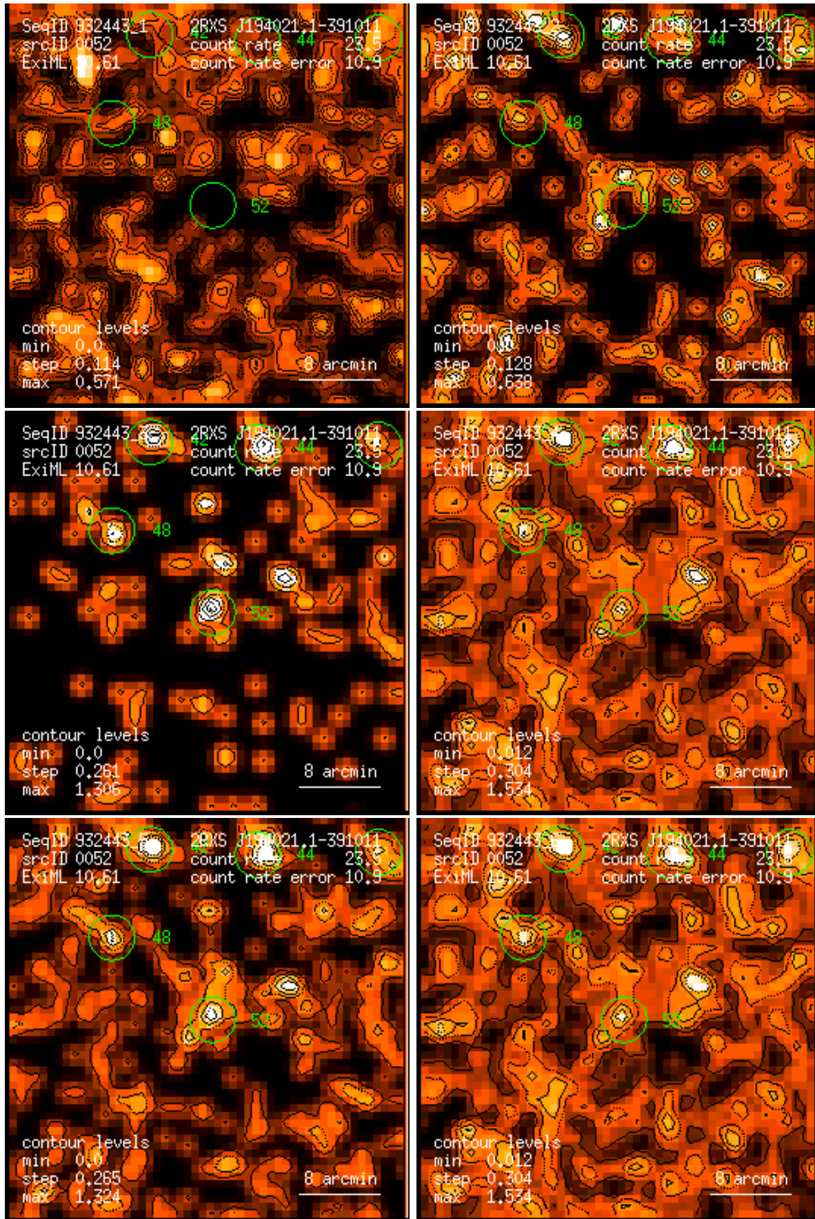
Figure 52: RASS 932443: detection 0052: band rate images, Gaussian filter: (1) PSPC channels 11 – 41, (2) 52 – 90, (3) 91 – 201, (4) 11 – 235, (5) 52 – 201, (6) 11 – 201. Broad band rates in counts/ks. Band rate contour levels in counts/ks/arcmin 2 .
