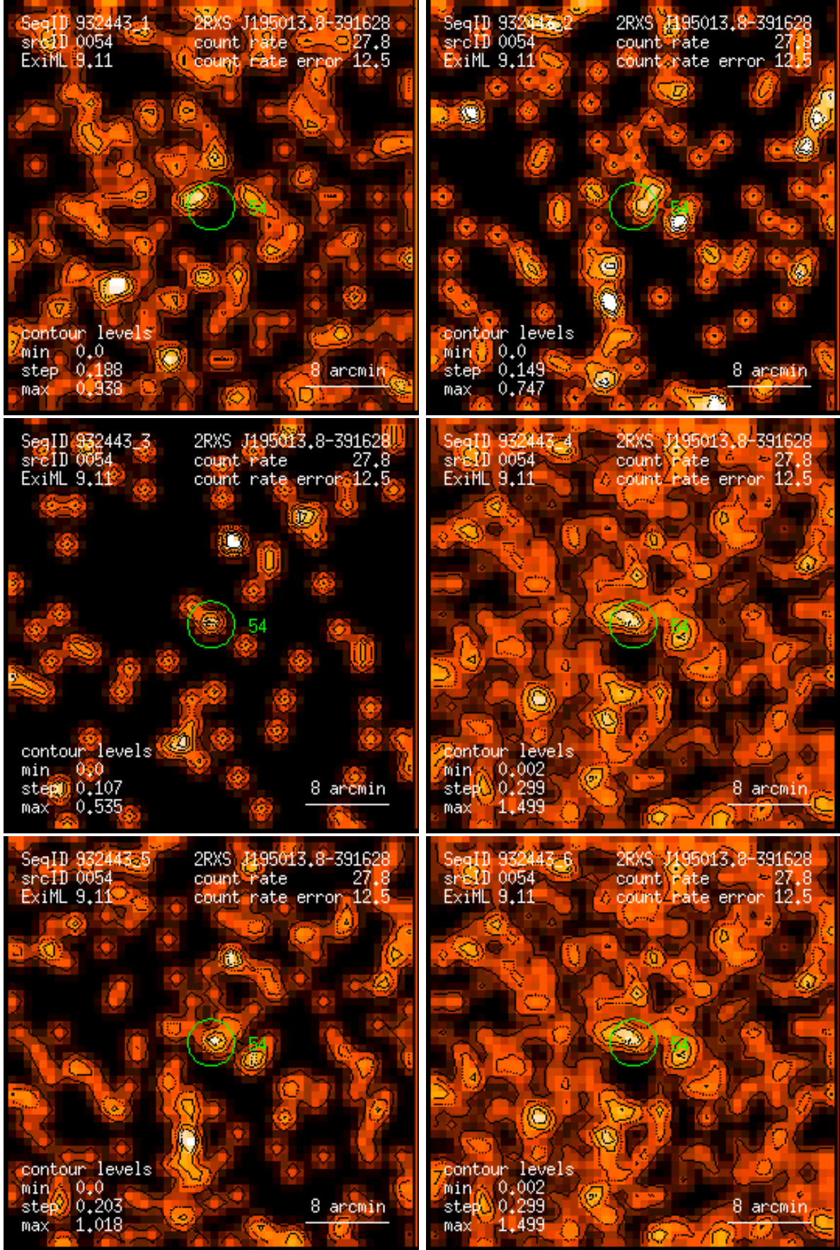
Figure 54: RASS 932443: detection 0054: band rate images, Gaussian filter: (1) PSPC channels 11 – 41, (2) 52 – 90, (3) 91 – 201, (4) 11 – 235, (5) 52 – 201, (6) 11 – 201. Broad band rates in counts/ks. Band rate contour levels in counts/ks/arcmin 2 .
