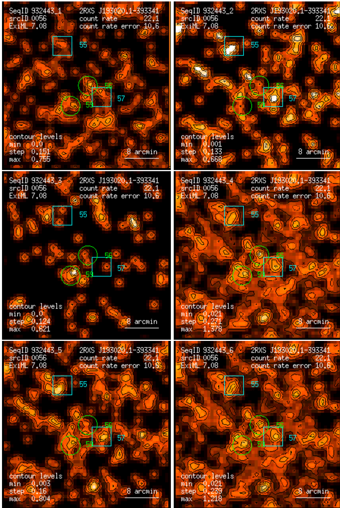
Figure 56: RASS 932443: detection 0056: band rate images, Gaussian filter: (1) PSPC channels 11 – 41, (2) 52 – 90, (3) 91 – 201, (4) 11 – 235, (5) 52 – 201, (6) 11 – 201. Broad band rates in counts/ks. Band rate contour levels in counts/ks/arcmin 2 .
