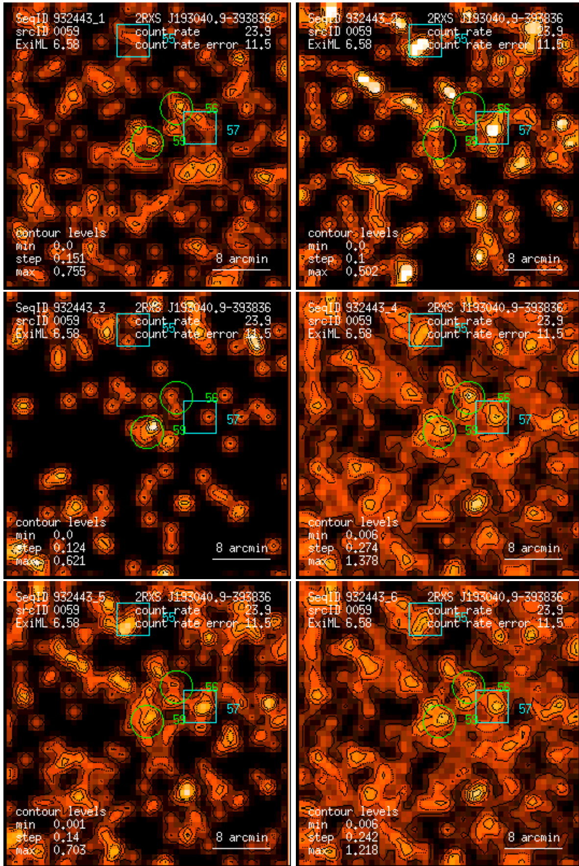
Figure 59: RASS 932443: detection 0059: band rate images, Gaussian filter: (1) PSPC channels 11 – 41, (2) 52 – 90, (3) 91 – 201, (4) 11 – 235, (5) 52 – 201, (6) 11 – 201. Broad band rates in counts/ks. Band rate contour levels in counts/ks/arcmin 2 .
