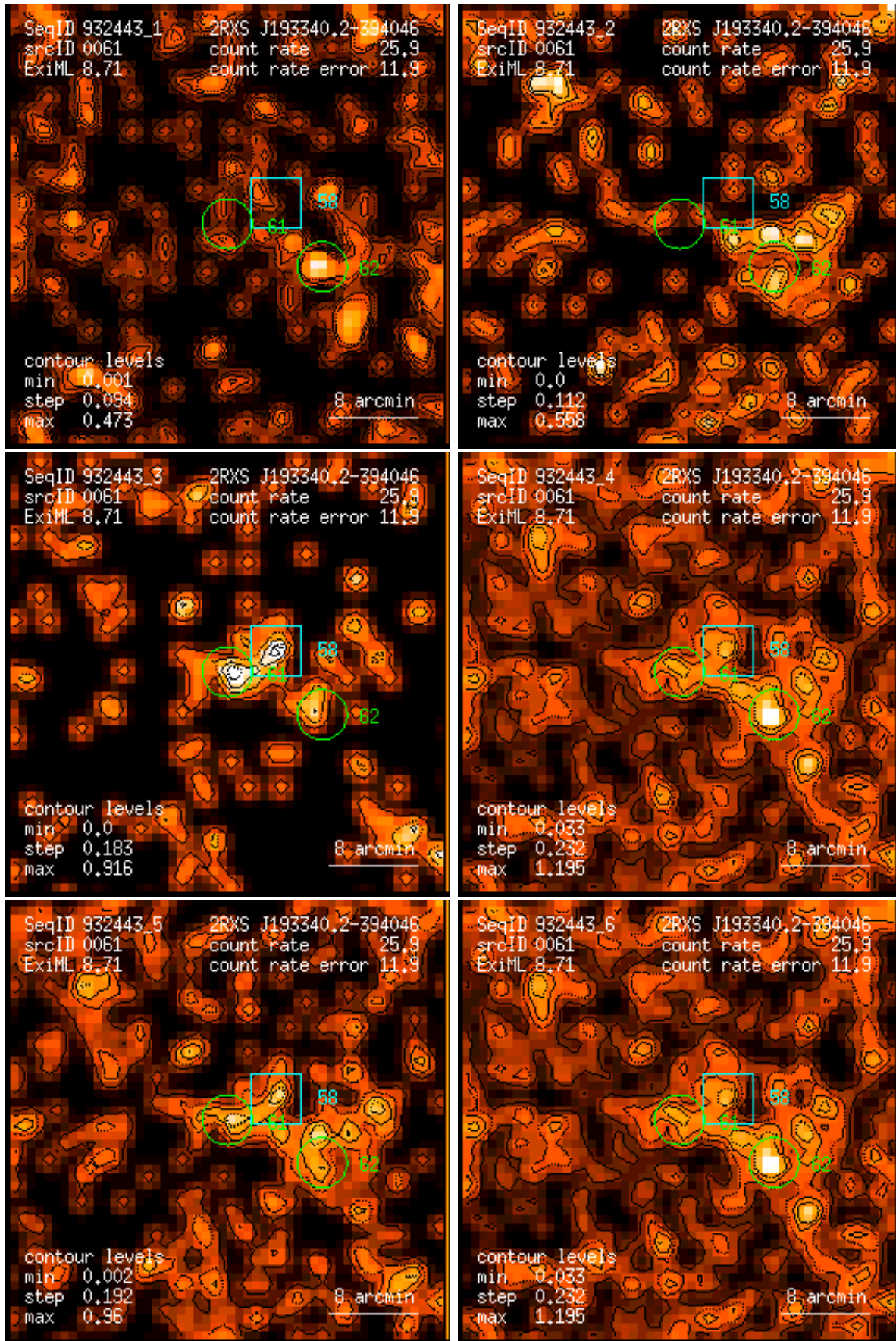
Figure 61: RASS 932443: detection 0061: band rate images, Gaussian filter: (1) PSPC channels 11 – 41, (2) 52 – 90, (3) 91 – 201, (4) 11 – 235, (5) 52 – 201, (6) 11 – 201. Broad band rates in counts/ks. Band rate contour levels in counts/ks/arcmin 2 .
