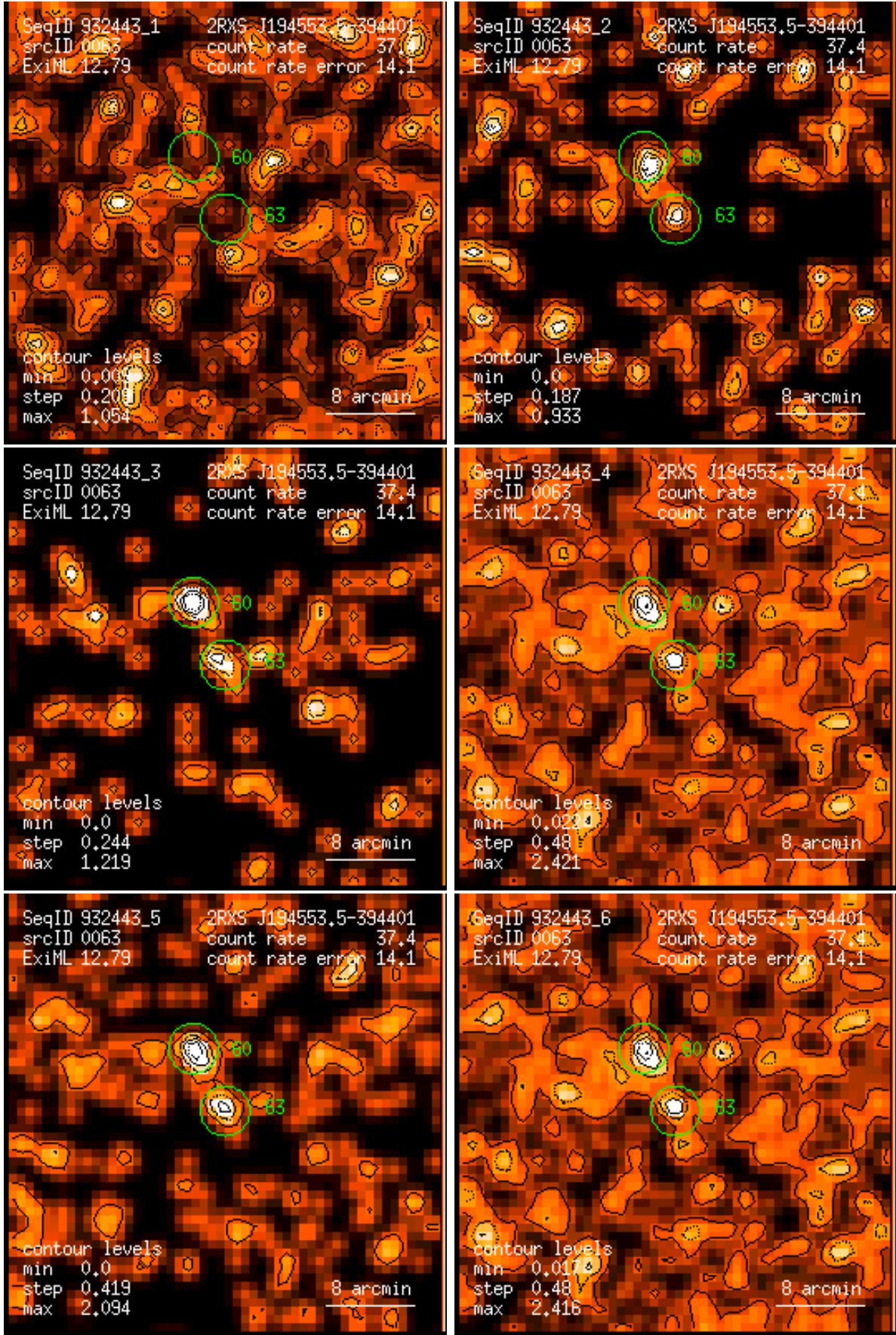
Figure 63: RASS 932443: detection 0063: band rate images, Gaussian filter: (1) PSPC channels 11 – 41, (2) 52 – 90, (3) 91 – 201, (4) 11 – 235, (5) 52 – 201, (6) 11 – 201. Broad band rates in counts/ks. Band rate contour levels in counts/ks/arcmin 2 .
