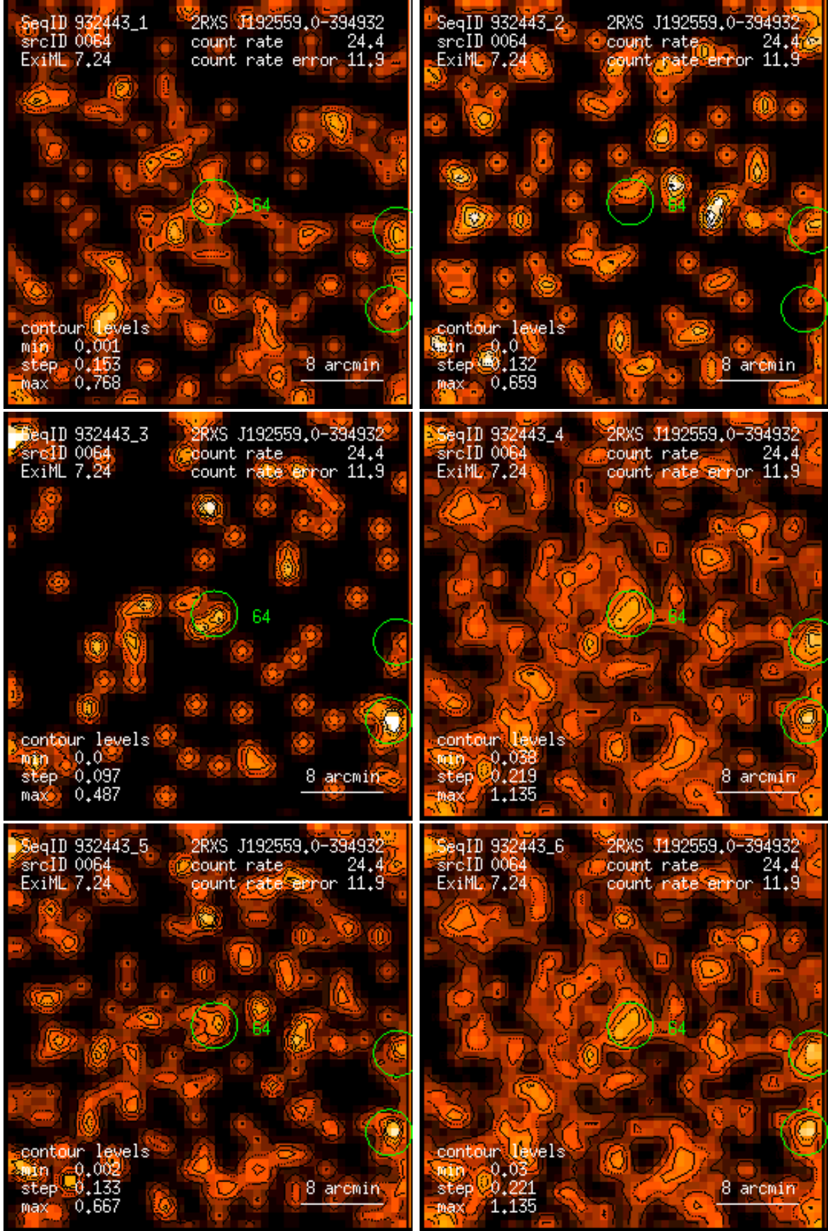
Figure 64: RASS 932443: detection 0064: band rate images, Gaussian filter: (1) PSPC channels 11 – 41, (2) 52 – 90, (3) 91 – 201, (4) 11 – 235, (5) 52 – 201, (6) 11 – 201. Broad band rates in counts/ks. Band rate contour levels in counts/ks/arcmin 2 .
