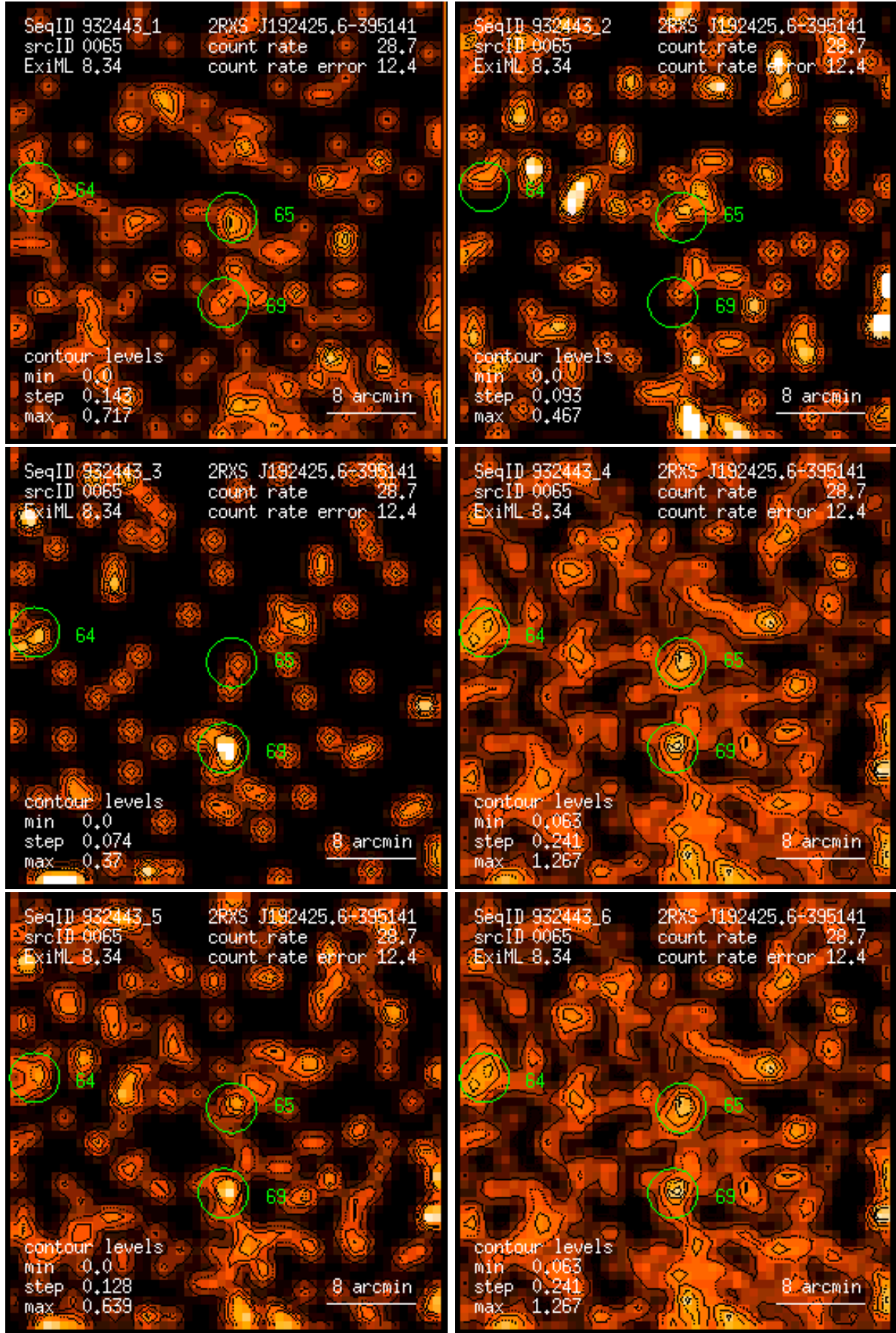
Figure 65: RASS 932443: detection 0065: band rate images, Gaussian filter: (1) PSPC channels 11 – 41, (2) 52 – 90, (3) 91 – 201, (4) 11 – 235, (5) 52 – 201, (6) 11 – 201. Broad band rates in counts/ks. Band rate contour levels in counts/ks/arcmin 2 .
